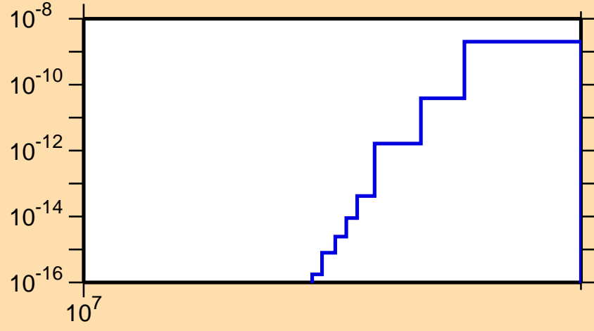
\sigma vs. E for ^{124}\text{Ce} (mt 34)
