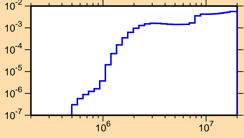
\sigma vs. E for ^{124}\text{Ce}(n,n\text{cont.})
