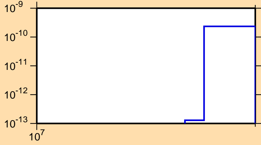
\sigma vs. E for ^{124}\text{Ce}(n,2n\alpha)
