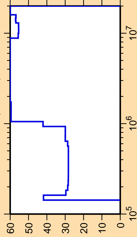
\Delta\sigma/\sigma vs. E for ^{124}\text{Ce}(n,\text{inel.})
