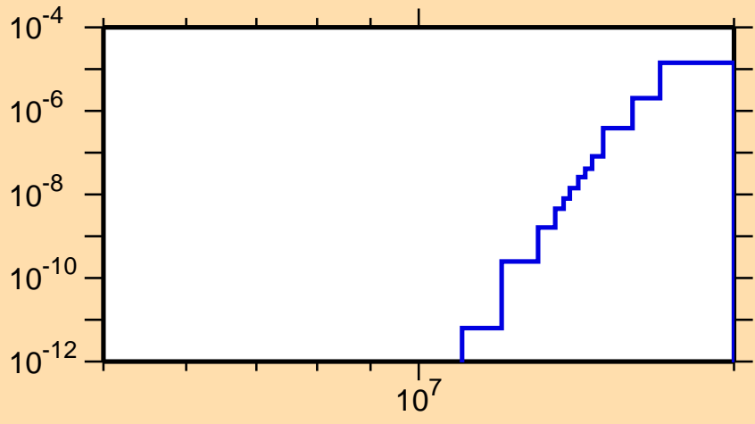
\sigma vs. E for ^{124}\text{Ce} (mt 45)
