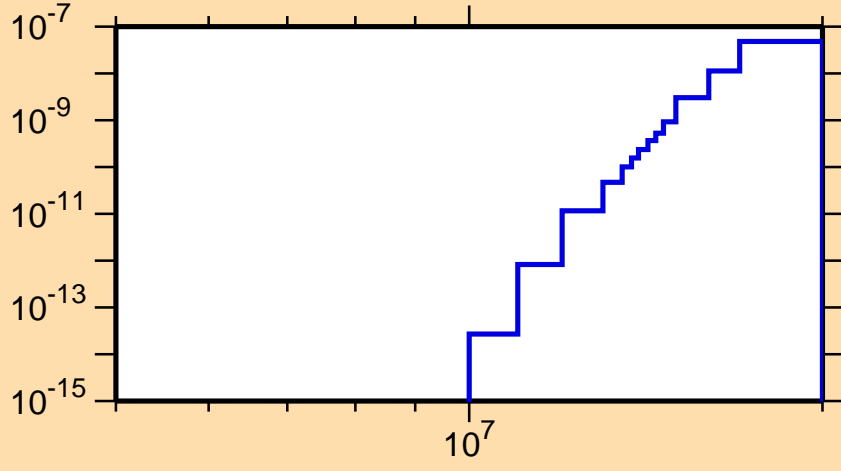
\sigma vs. E for ^{124}\text{Ce}(\text{mt117})
