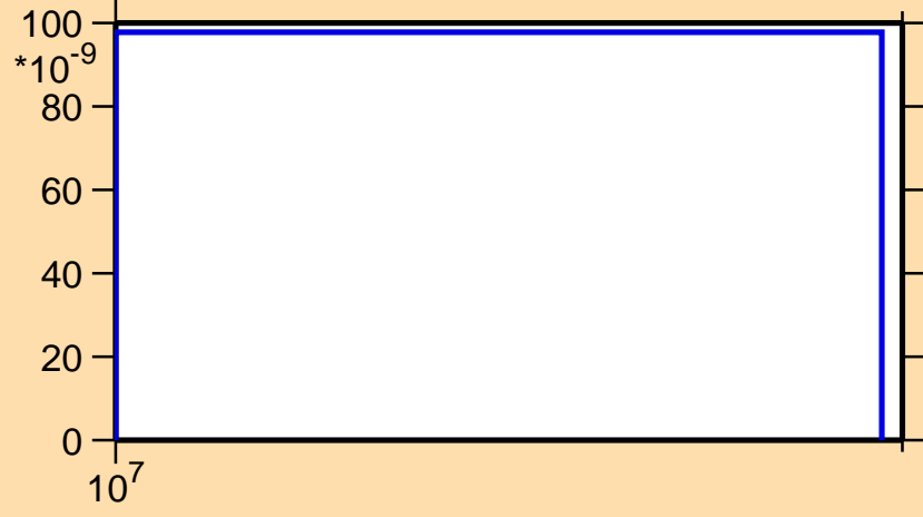
\sigma vs. E for ^{124}\text{Ce}(n,\text{pt})
