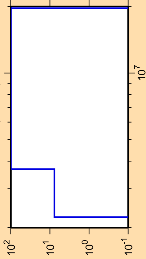
\Delta\sigma/\sigma vs. E for ^{124}\text{Ce}(n,\text{He}3)
