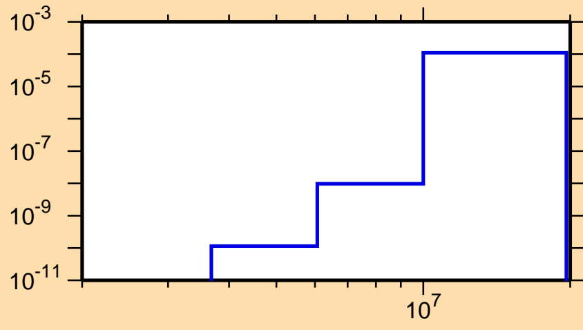
\sigma vs. E for ^{124}\text{Ce}(n,\text{He}3)
