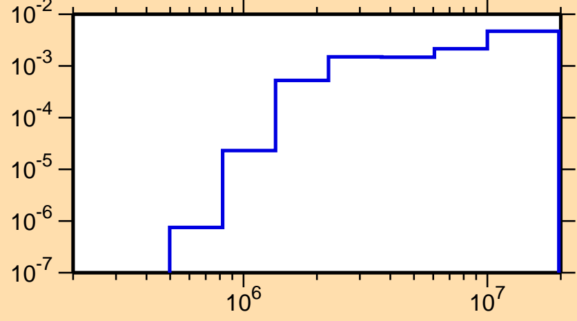
\sigma vs. E for ^{124}\text{Ce}(n,n\text{cont.})
