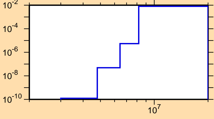
\sigma vs. E for ^{124}\text{Ce}(n,d)
