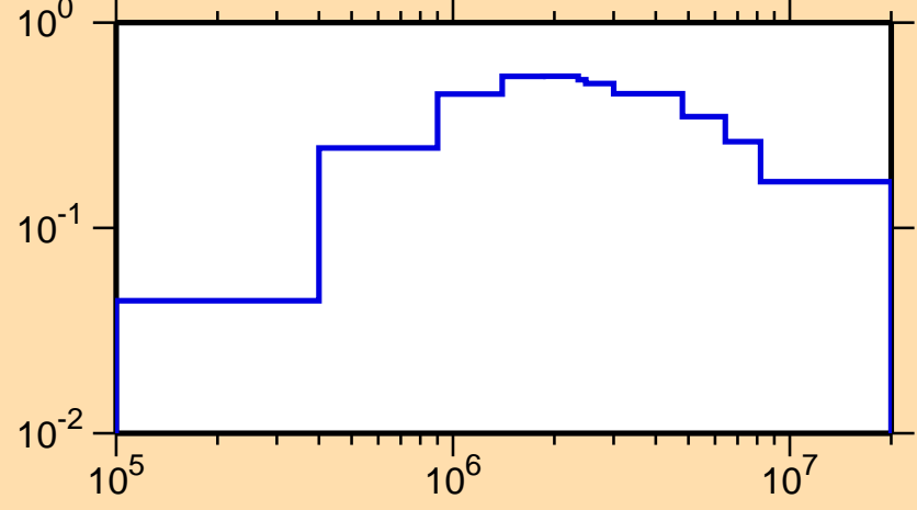
\sigma vs. E for ^{124}\text{Ce}(n,\text{inel.})
