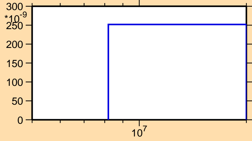
\sigma vs. E for ^{124}\text{Ce} (mt 45)
