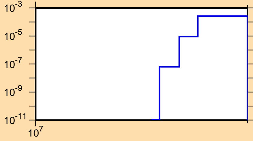
\sigma vs. E for ^{125}\text{Ce}(n,2np)
