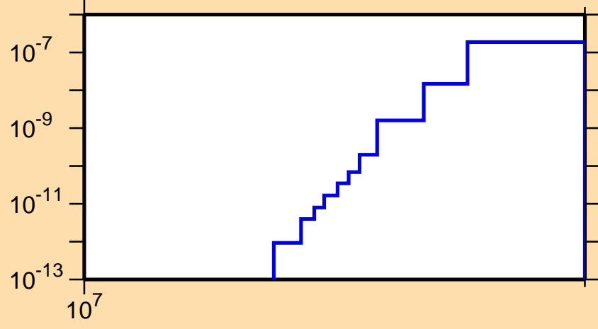
\sigma vs. E for ^{125}\text{Ce} (mt 34)
