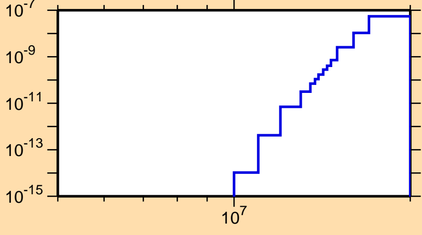
\sigma vs. E for ^{125}\text{Ce}(\text{mt117})
