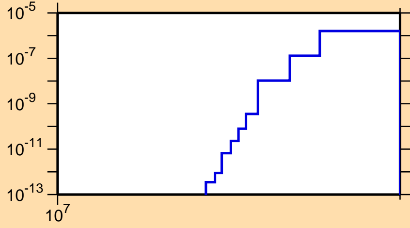
\sigma vs. E for ^{125}\text{Ce}(n,\text{nd})
