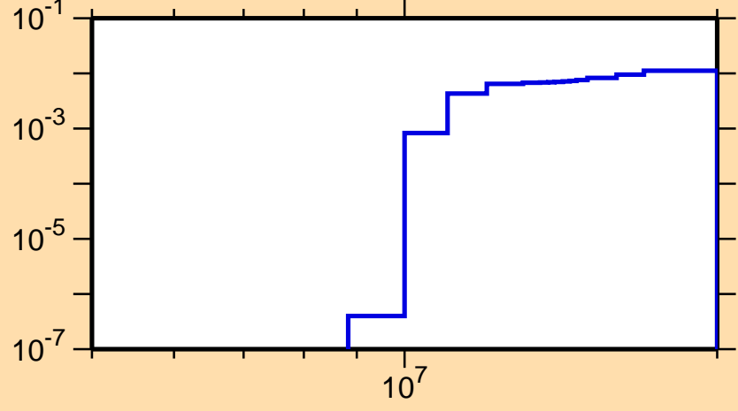
\sigma vs. E for ^{125}\text{Ce}(n,2n)
