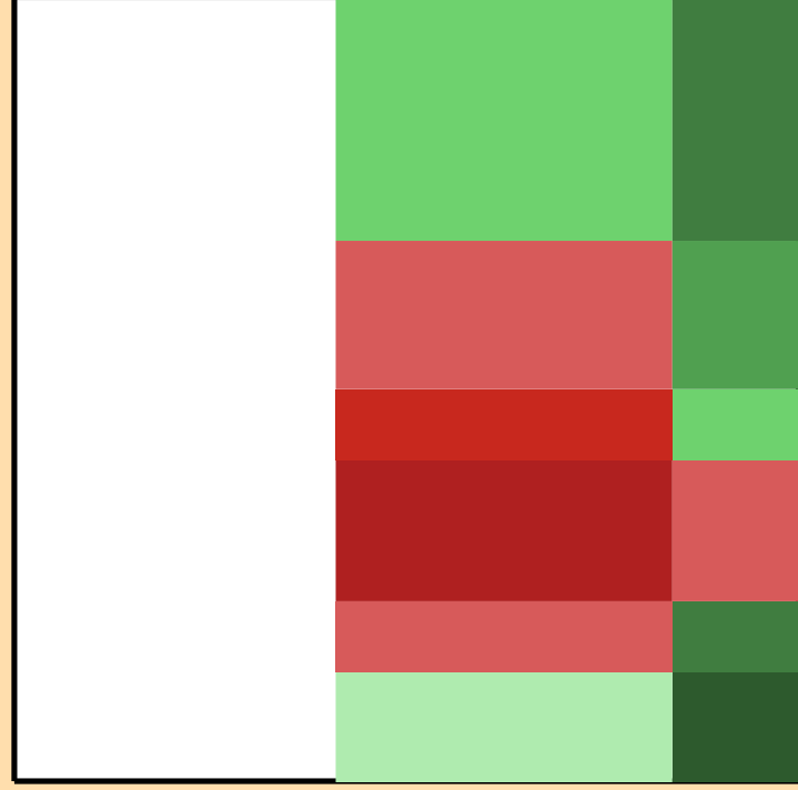
\Delta\sigma/\sigma vs. E for ^{125}\text{Ce}(n,2n)
