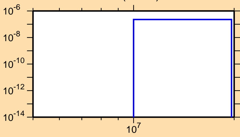
\sigma vs. E for ^{125}\text{Ce}(\text{mt } 45)
