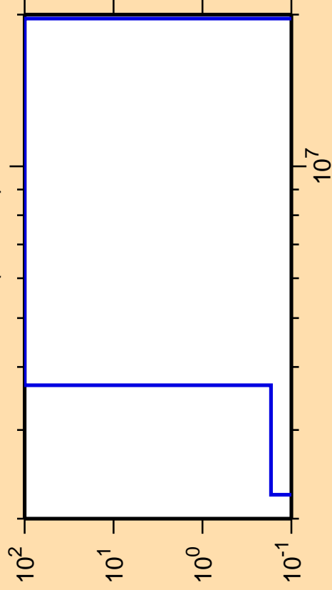
\Delta\sigma/\sigma vs. E for ^{125}\text{Ce}(n,\text{He3})
