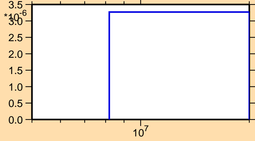
\sigma vs. E for ^{125}\text{Ce}(n,\text{pt})
