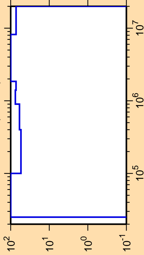
\Delta\sigma/\sigma vs. E for ^{125}\text{Ce}(n,\text{inel.})
