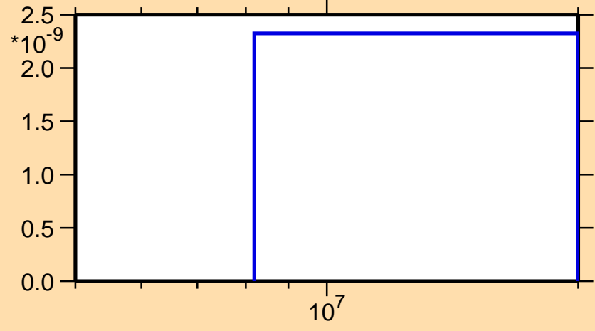
\sigma vs. E for ^{125}\text{Ce}(n,2n\alpha)
