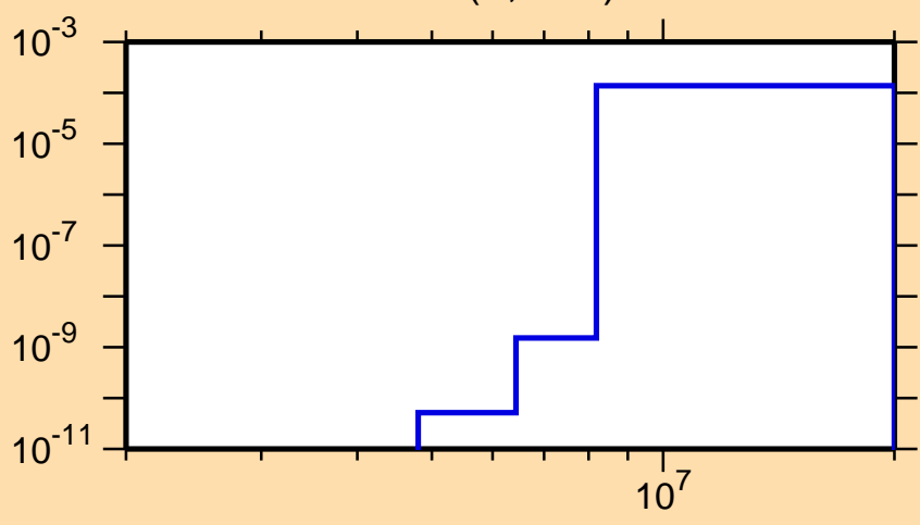
\sigma vs. E for ^{125}\text{Ce}(n,\text{He}3)
