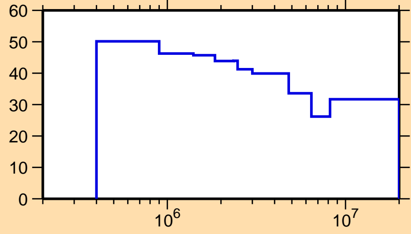
\Delta\sigma/\sigma vs. E for ^{125}\text{Ce}(n,n\text{onel.})
