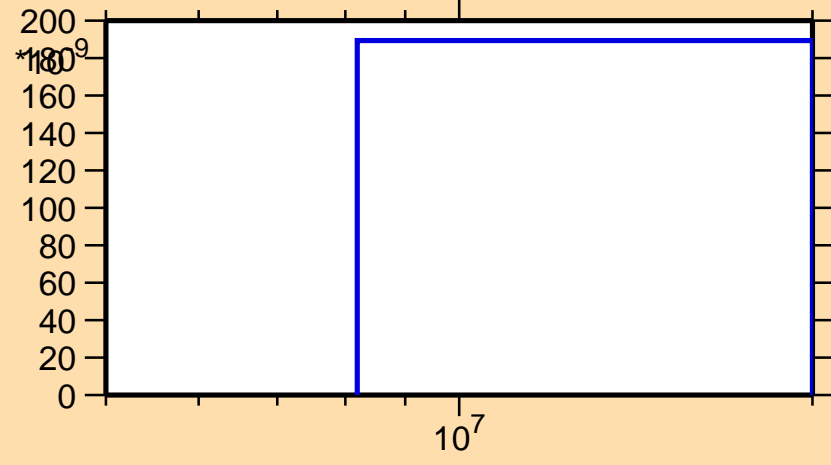
\sigma vs. E for ^{125}\text{Ce}(\text{mt } 45)
