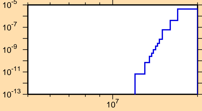
\sigma vs. E for ^{126}\text{Ce} (mt 45)
