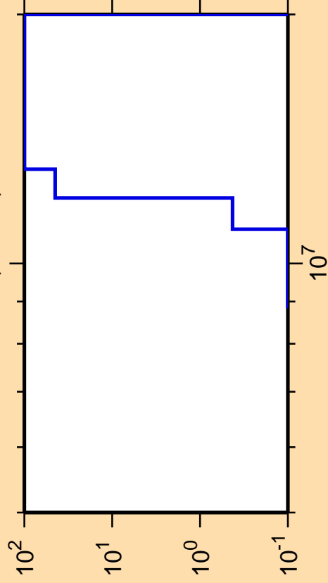
\Delta\sigma/\sigma vs. E for ^{126}\text{Ce} (mt 45)
