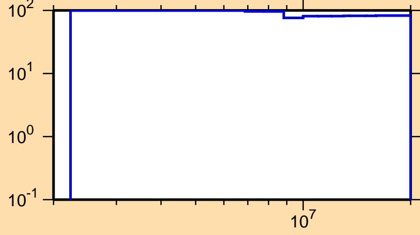
\Delta\sigma/\sigma vs. E for ^{126}\text{Ce}(n,n\text{cont.})
