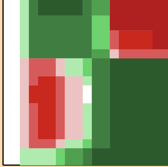
\Delta\sigma/\sigma vs. E for ^{126}\text{Ce}(n,n\text{cont.})
