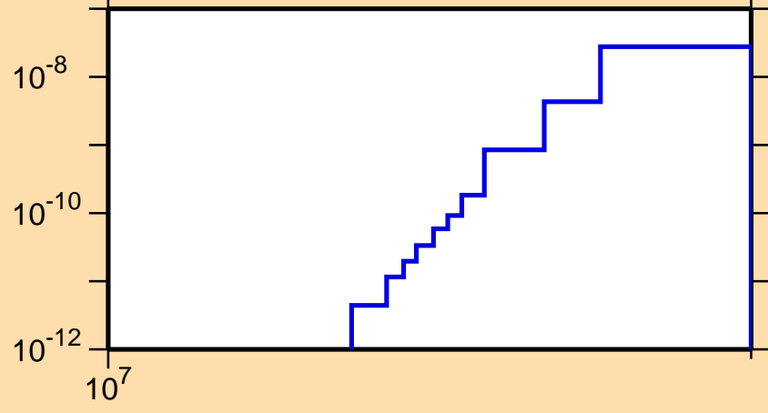
\sigma vs. E for ^{126}\text{Ce}(\text{mt117})
