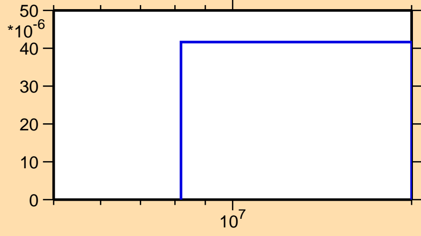
\sigma vs. E for ^{126}\text{Ce}(n,\text{pd})
