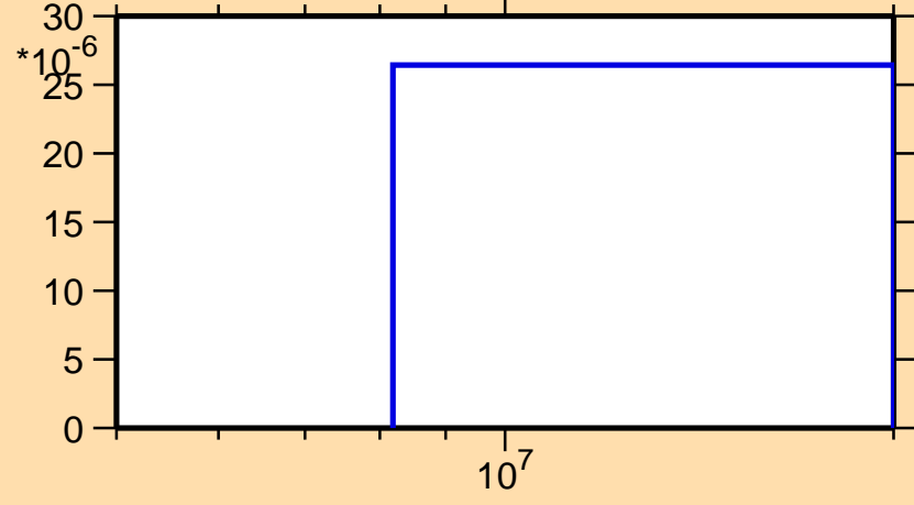
\sigma vs. E for ^{126}\text{Ce}(n,t)
