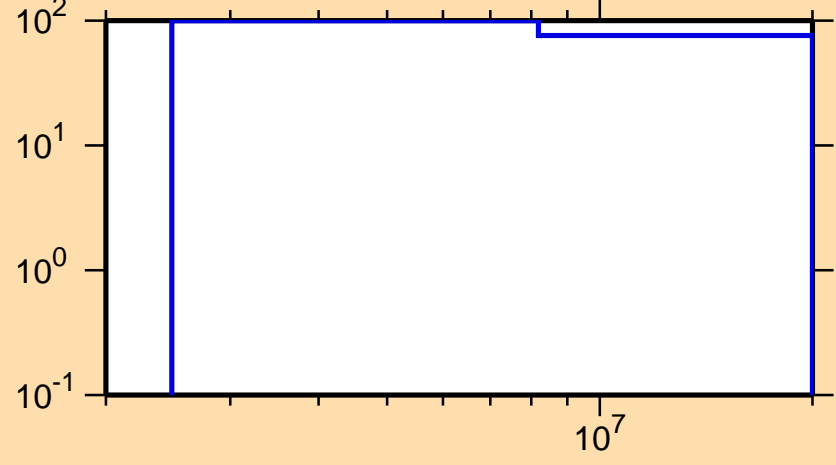
\Delta\sigma/\sigma vs. E for ^{126}\text{Ce}(n,ncont.)
