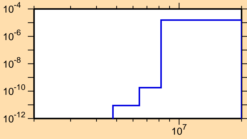
\sigma vs. E for ^{126}\text{Ce}(n,\text{He3})
