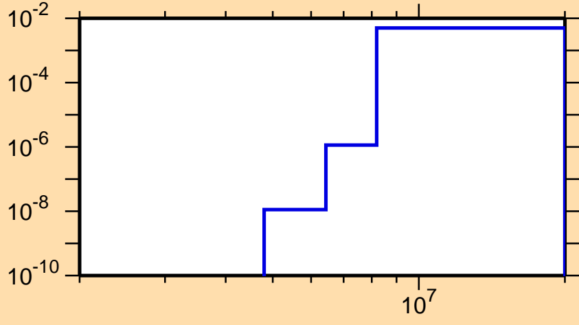
\sigma vs. E for ^{126}\text{Ce}(n,d)
