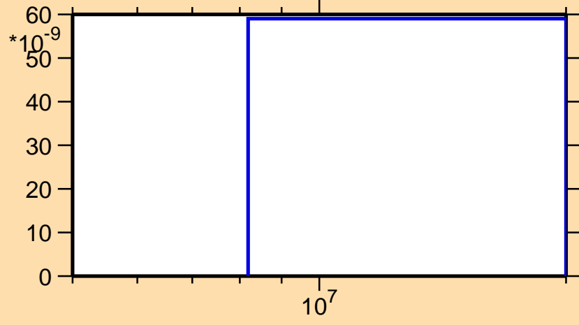
\sigma vs. E for ^{126}\text{Ce} (mt 45)
