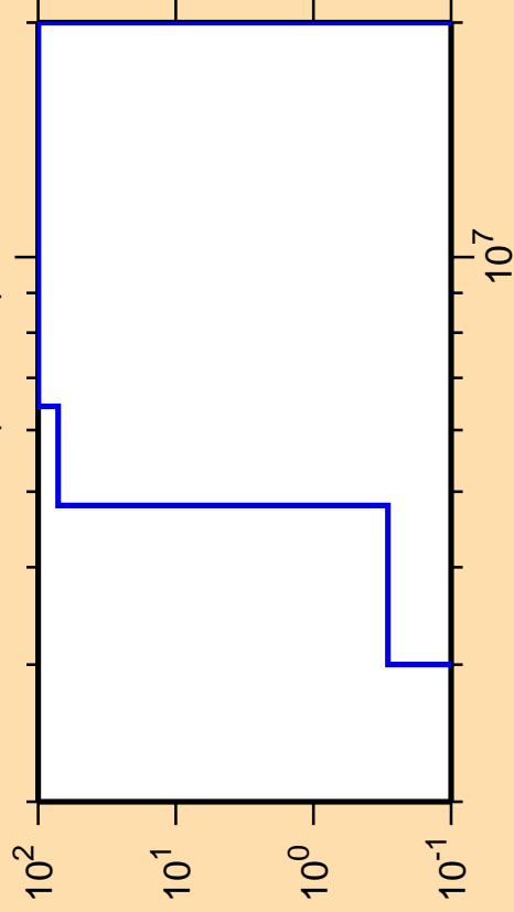
\Delta\sigma/\sigma vs. E for ^{126}\text{Ce}(n,\text{He3})
