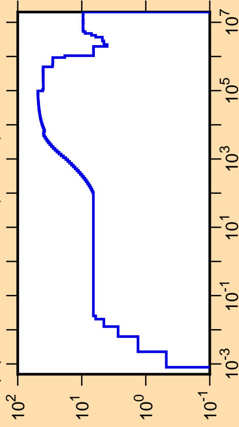
\Delta\mu/\mu vs. E for ^{127}\text{Ce}(\text{mt251})
