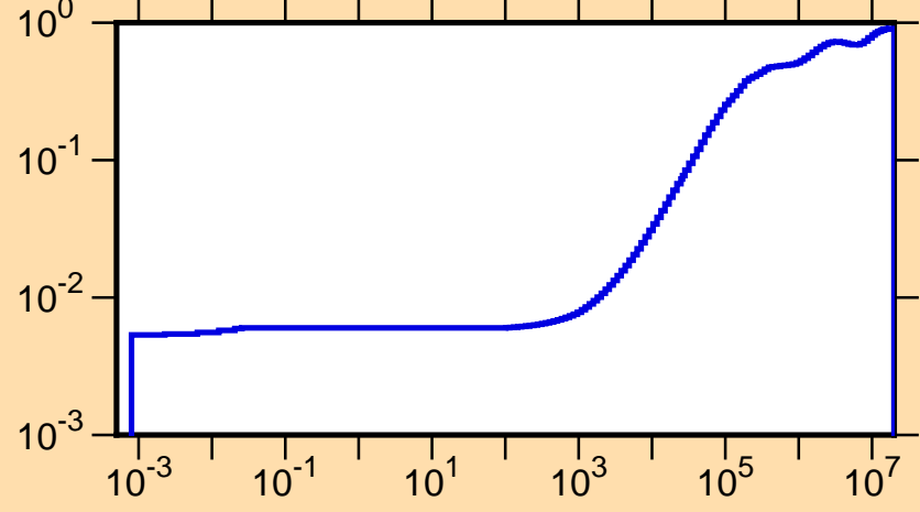
\mu vs. E for ^{127}\text{Ce}(\text{mt251})
