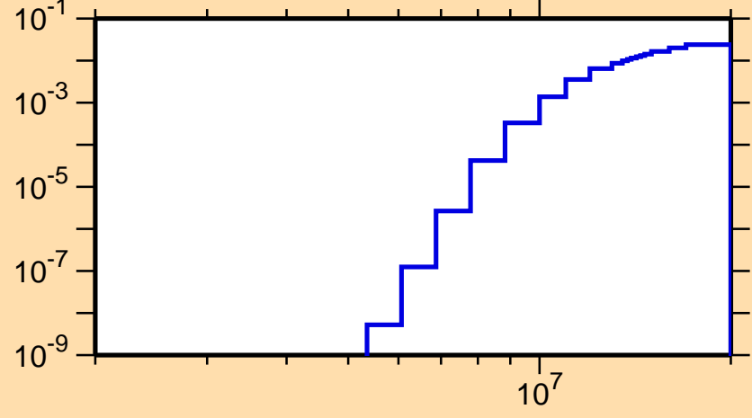
\sigma vs. E for ^{127}\text{Ce}(n,d)
