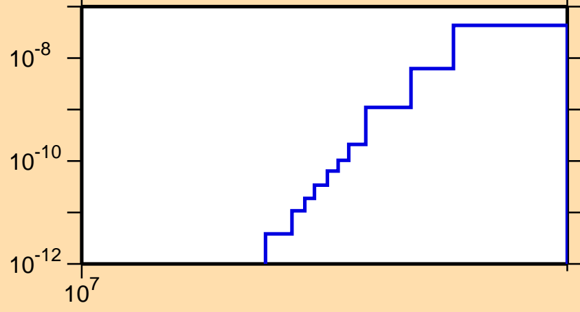
\sigma vs. E for ^{127}\text{Ce}(\text{mt117})
