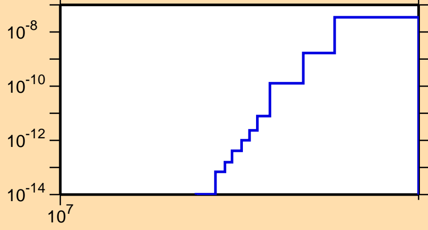
\sigma vs. E for ^{127}\text{Ce} (mt 34)
