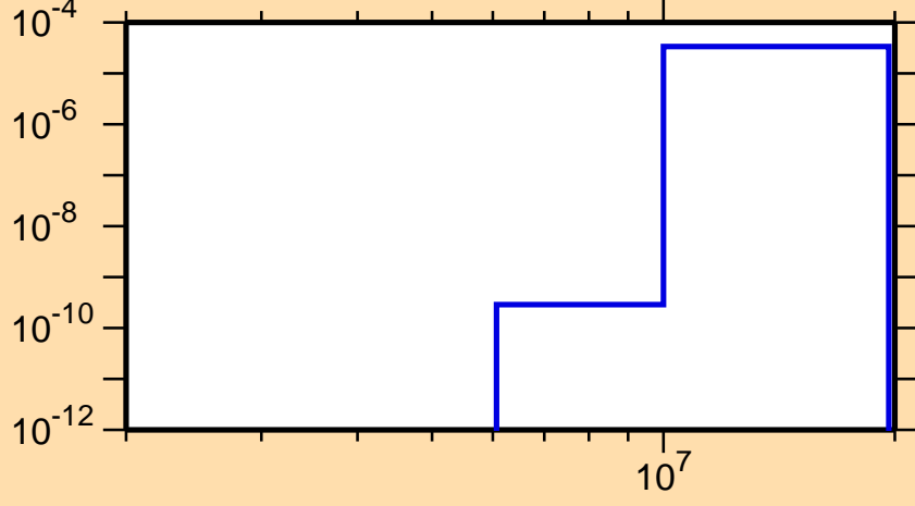
\sigma vs. E for ^{127}\text{Ce}(n,\text{He}3)
