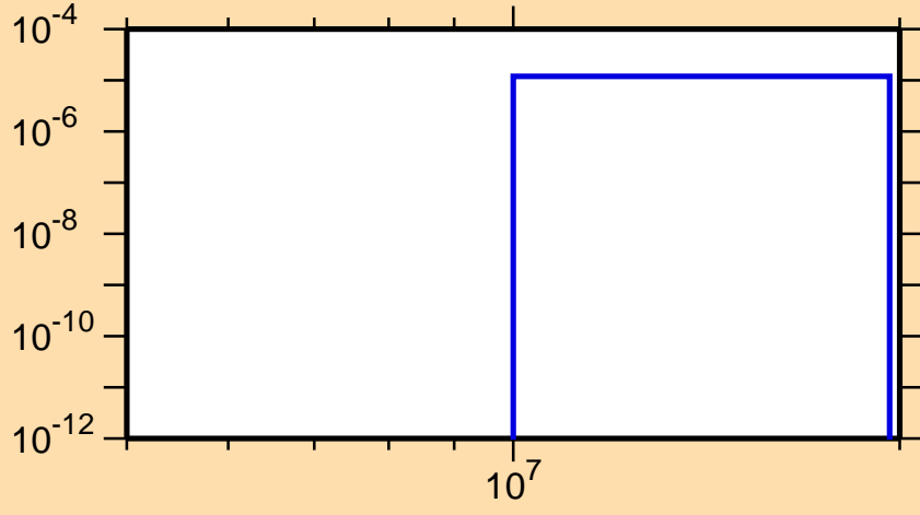
\sigma vs. E for ^{127}\text{Ce}(n,\text{pd})
