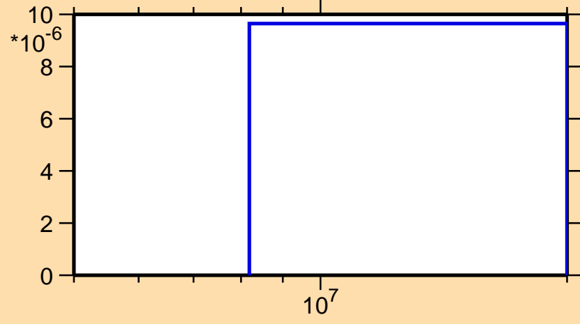
\sigma vs. E for ^{127}\text{Ce}(n,\text{pd})
