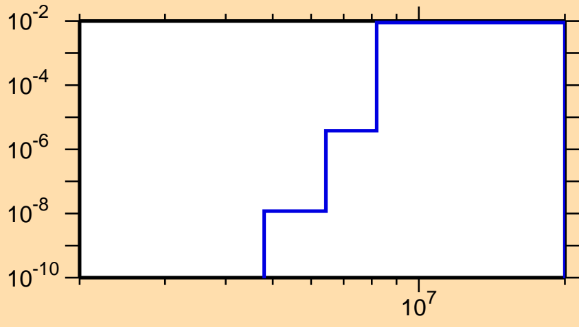
\sigma vs. E for ^{127}\text{Ce}(n,d)
