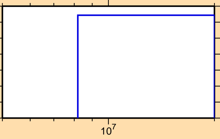
\sigma vs. E for ^{127}\text{Ce}(n,\text{pt})
