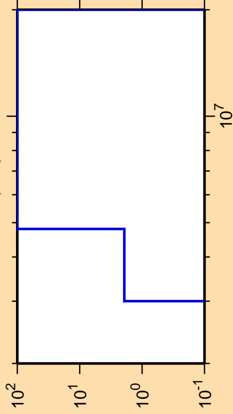
\Delta\sigma/\sigma vs. E for ^{127}\text{Ce}(n,d)
