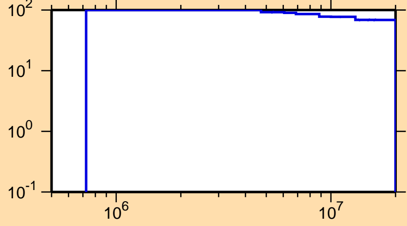
\Delta\sigma/\sigma vs. E for ^{127}\text{Ce}(n,ncont.)
