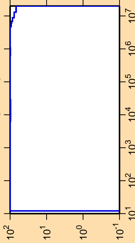
\Delta\sigma/\sigma vs. E for ^{127}\text{Ce}(n,\text{inel.})
