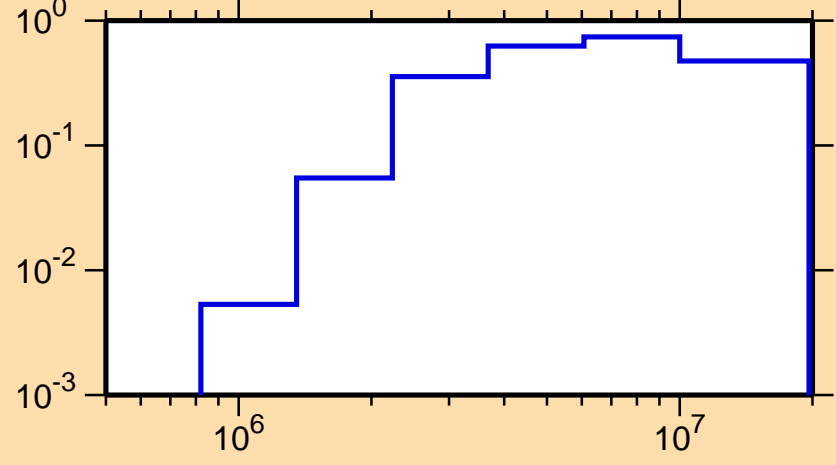
\sigma vs. E for ^{127}\text{Ce}(n,n\text{cont.})
