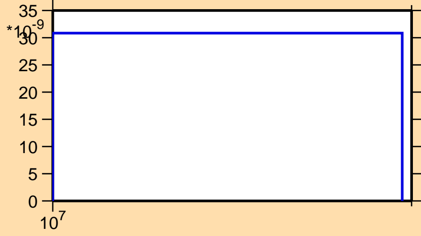
\sigma vs. E for ^{127}\text{Ce} (mt 45)
