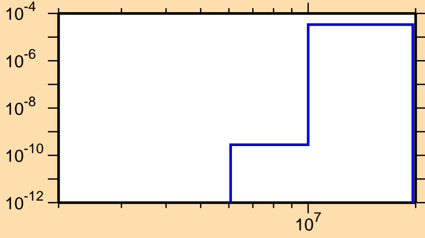
\sigma vs. E for ^{127}\text{Ce}(n,\text{He}3)
