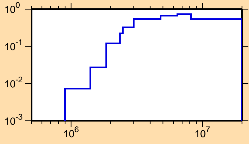
\sigma vs. E for ^{127}\text{Ce}(n,n\text{cont.})
