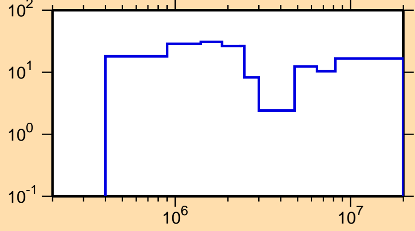
\Delta\sigma/\sigma vs. E for ^{127}\text{Ce}(n,\text{tot.})
