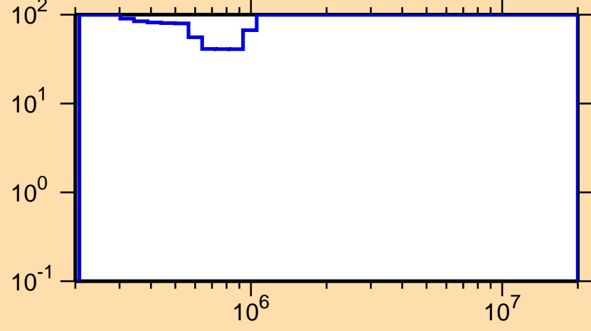
\Delta\sigma/\sigma vs. E for ^{128}\text{Ce}(n,n_1)
