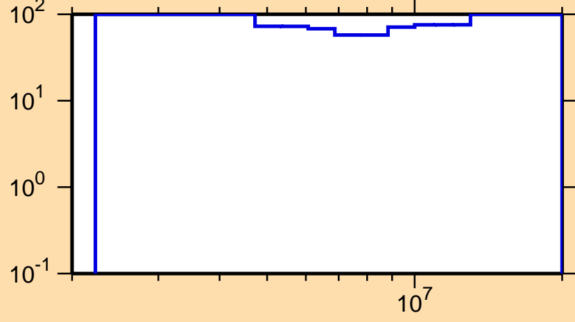
\Delta\sigma/\sigma vs. E for ^{128}\text{Ce}(n,n\text{cont.})
