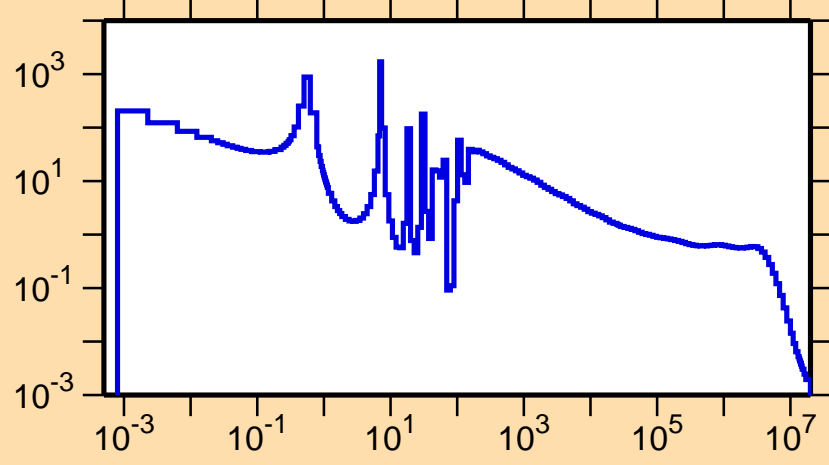
\sigma vs. E for ^{128}\text{Ce}(n,\gamma)
