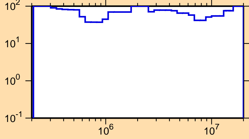
\Delta\sigma/\sigma vs. E for ^{128}\text{Ce}(n,\text{inel.})
