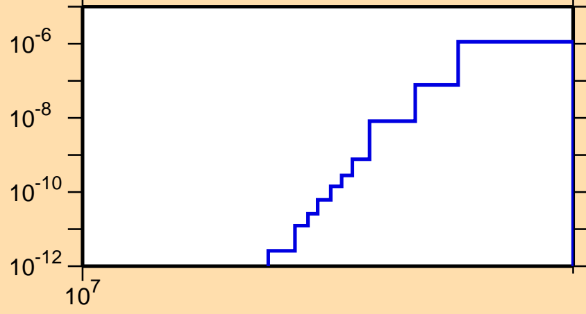
\sigma vs. E for ^{128}\text{Ce} (mt 45)
