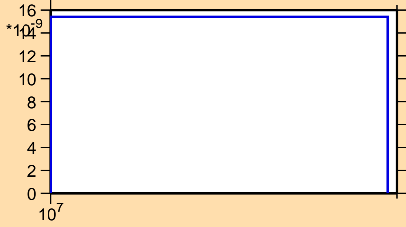
\sigma vs. E for ^{128}\text{Ce} (mt 45)
