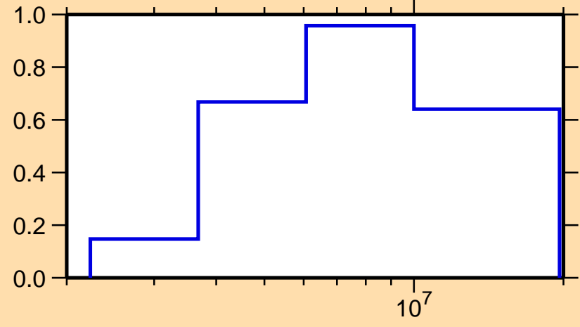
\sigma vs. E for ^{128}\text{Ce}(n,n\text{cont.})
