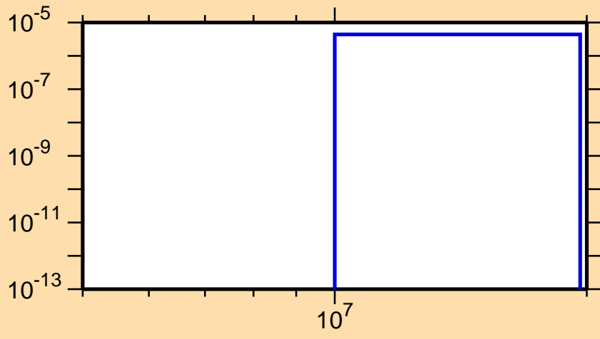
\sigma vs. E for ^{128}\text{Ce}(n,pd)
