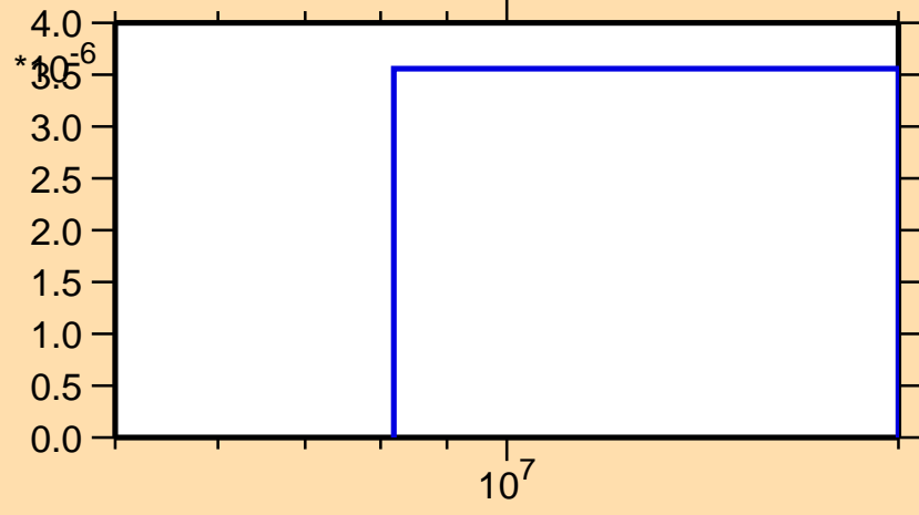
\sigma vs. E for ^{128}\text{Ce}(n,\text{pd})
