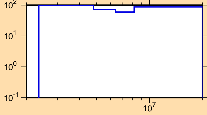
\Delta\sigma/\sigma vs. E for ^{128}\text{Ce}(n,n\text{cont.})
