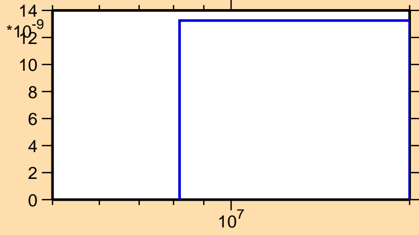
\sigma vs. E for ^{128}\text{Ce} (mt 45)
