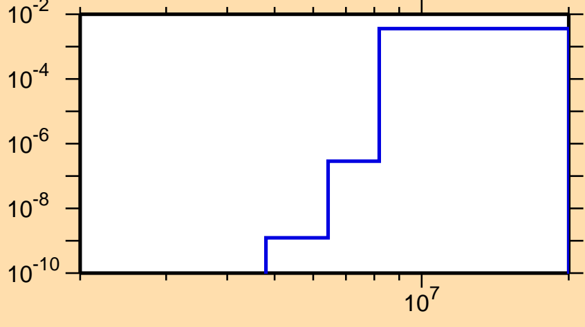
\sigma vs. E for ^{128}\text{Ce}(n,d)
