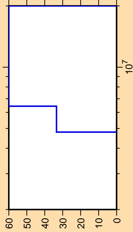
\Delta\sigma/\sigma vs. E for ^{128}\text{Ce}(n,np)
