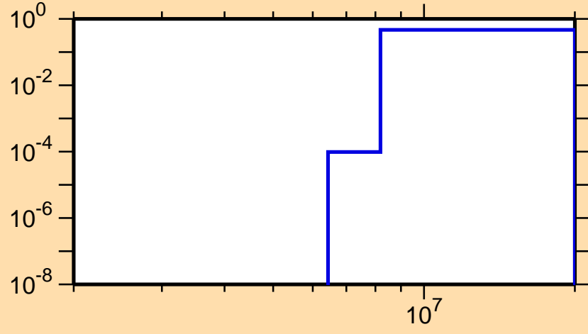
\sigma vs. E for ^{128}\text{Ce}(n,np)
