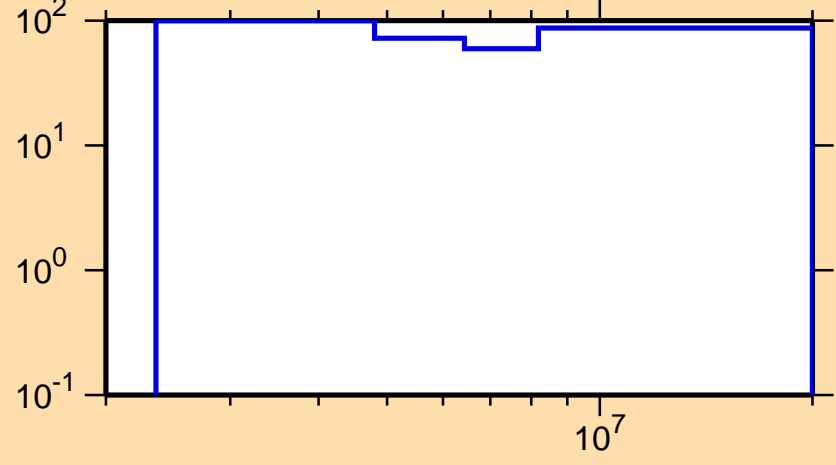
\Delta\sigma/\sigma vs. E for ^{128}\text{Ce}(n,ncont.)
