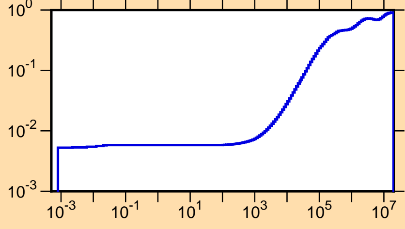
\mu vs. E for ^{129}\text{Ce}(\text{mt251})
