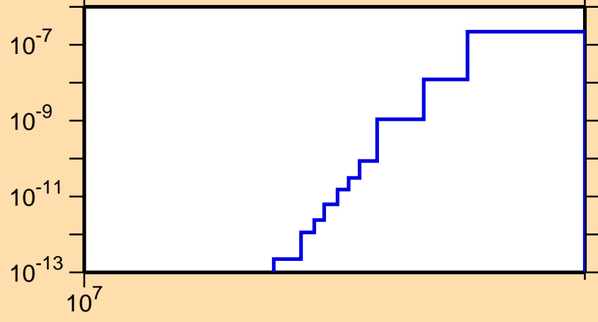
\sigma vs. E for ^{129}\text{Ce} (mt 45)
