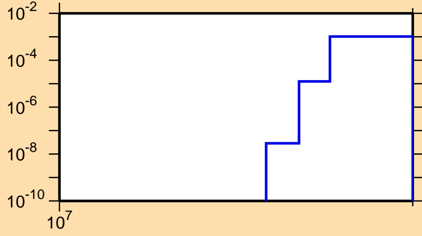
\sigma vs. E for ^{129}\text{Ce}(n,2np)
