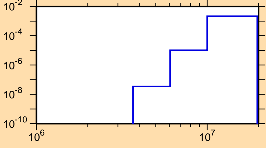
\sigma vs. E for ^{129}\text{Ce}(n,p\alpha)
