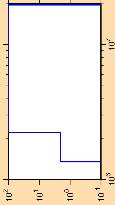
\Delta\sigma/\sigma vs. E for ^{129}\text{Ce}(n,p\alpha)
