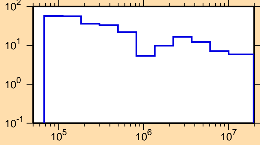
\Delta\sigma/\sigma vs. E for ^{129}\text{Ce}(n,\text{el.})
