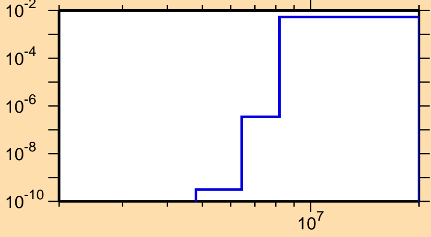
\sigma vs. E for ^{129}\text{Ce}(n,d)
