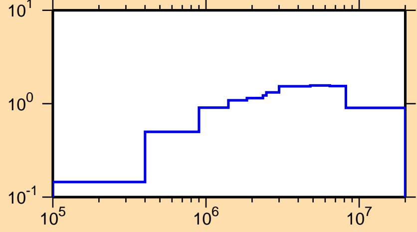
\sigma vs. E for ^{129}\text{Ce}(n,\text{inel.})
