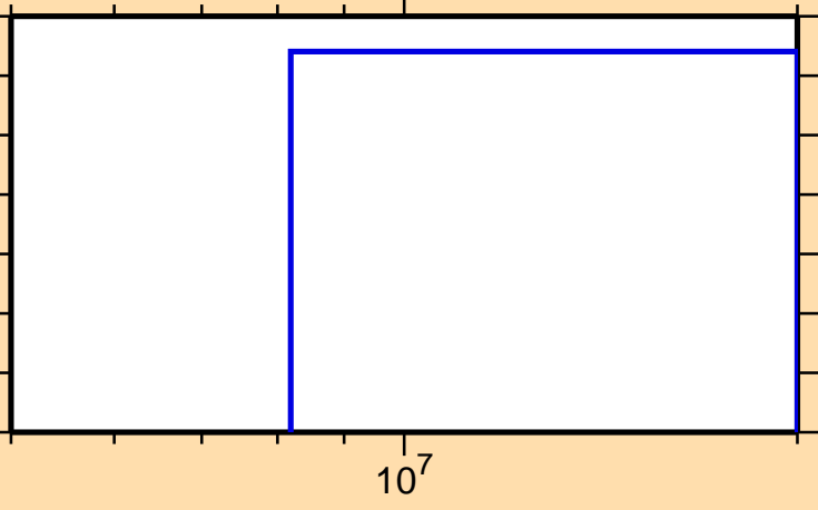
\sigma vs. E for ^{129}\text{Ce}(n,\text{pd})
