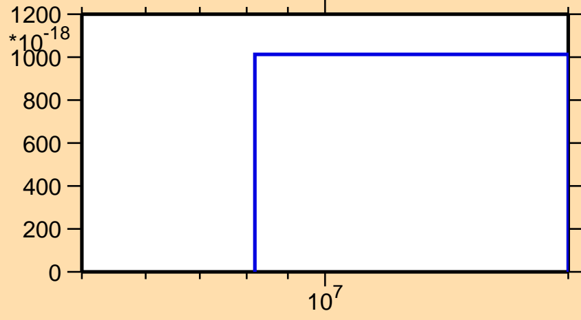
\sigma vs. E for ^{129}\text{Ce}(n,\text{nt})
