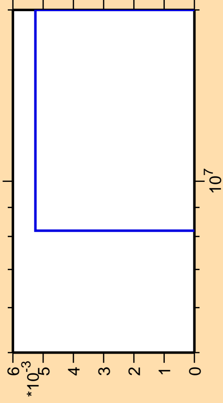
\Delta\sigma/\sigma vs. E for ^{129}\text{Ce}(n,\text{nt})
