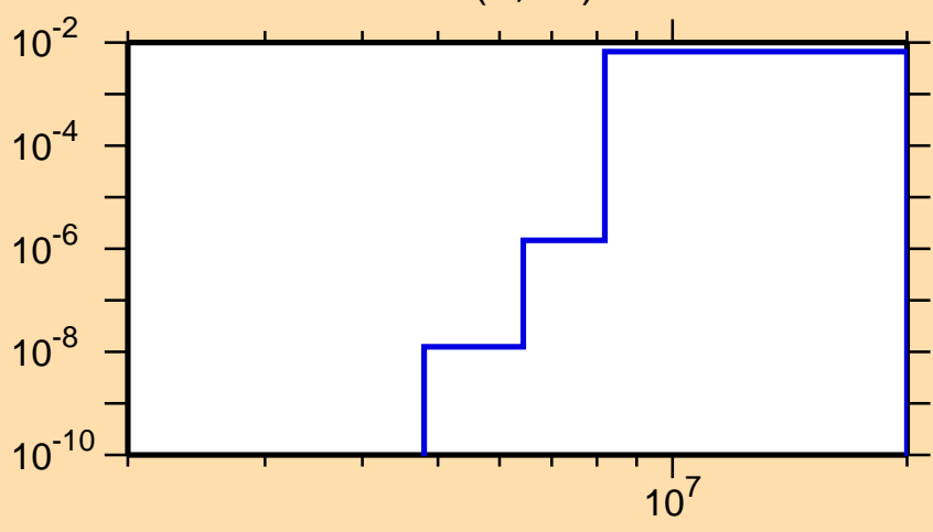
\sigma vs. E for ^{129}\text{Ce}(n,n\alpha)
