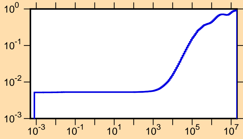
\mu vs. E for ^{130}\text{Ce}(\text{mt251})
