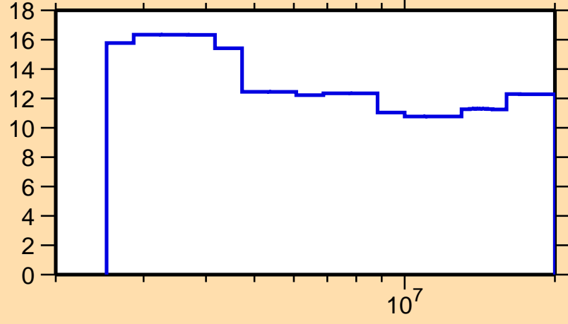
\Delta\sigma/\sigma vs. E for ^{130}\text{Ce}(n,n\text{onel.})
