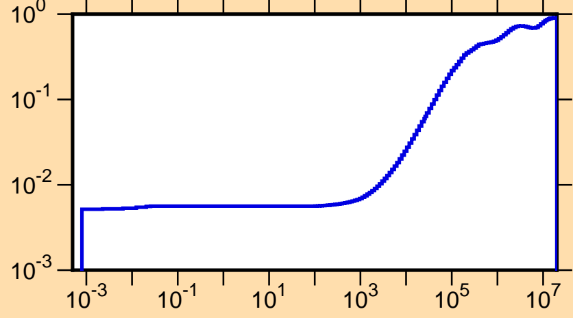
\mu vs. E for ^{131}\text{Ce}(\text{mt251})
