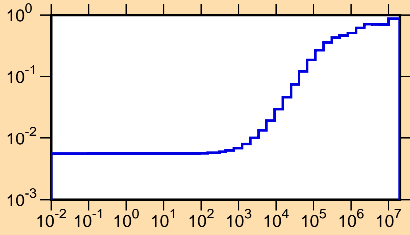
\mu vs. E for ^{131}\text{Ce}(\text{mt251})
