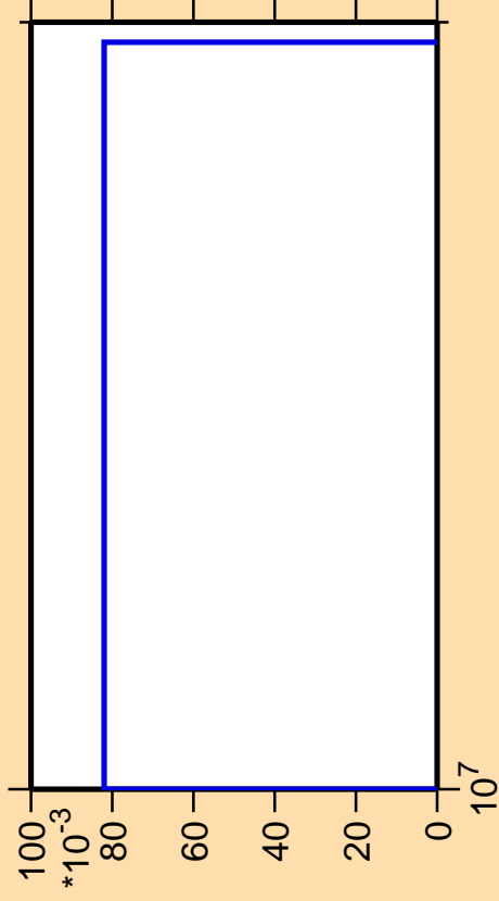
\Delta\sigma/\sigma vs. E for ^{131}\text{Ce}(n,\text{nt})
