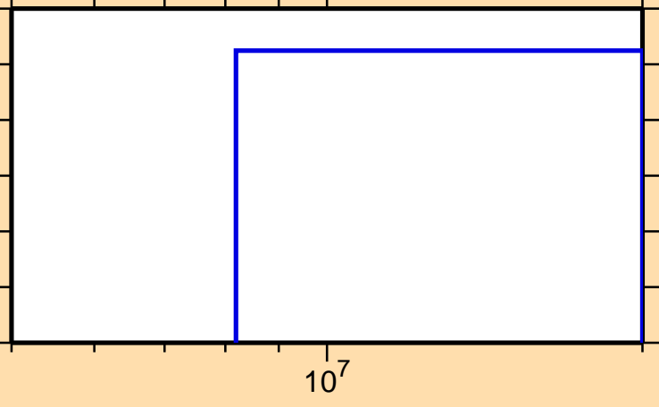
\sigma vs. E for ^{131}\text{Ce}(n,t)
