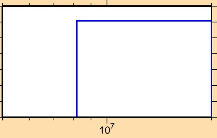
\sigma vs. E for ^{131}\text{Ce}(n,\text{He3})
