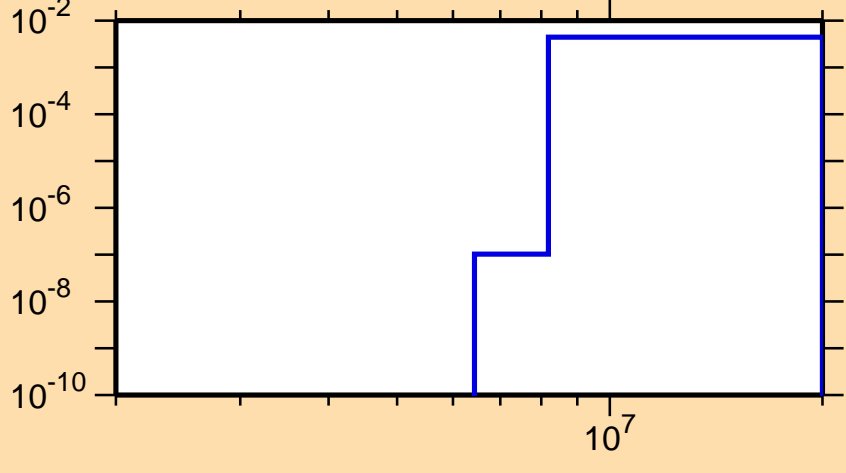
\sigma vs. E for ^{131}\text{Ce}(n,d)
