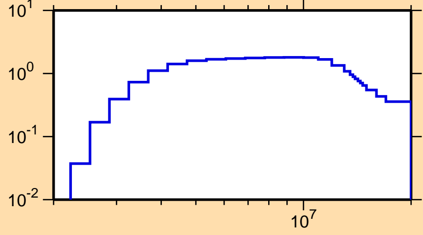
\sigma vs. E for ^{132}\text{Ce}(n,n\text{cont.})
