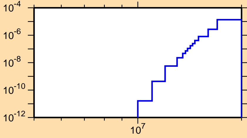
\sigma vs. E for ^{132}\text{Ce}(n,\text{He3})
