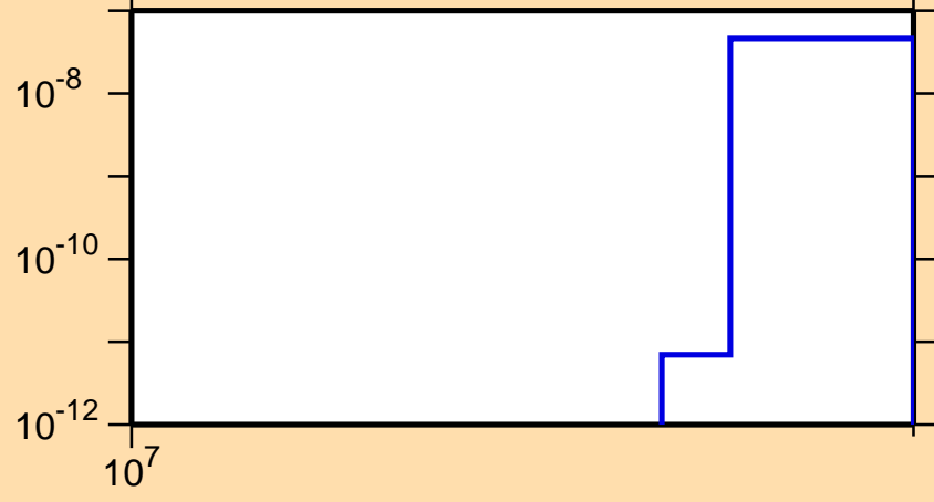
\sigma vs. E for ^{132}\text{Ce}(n,\text{nd})
