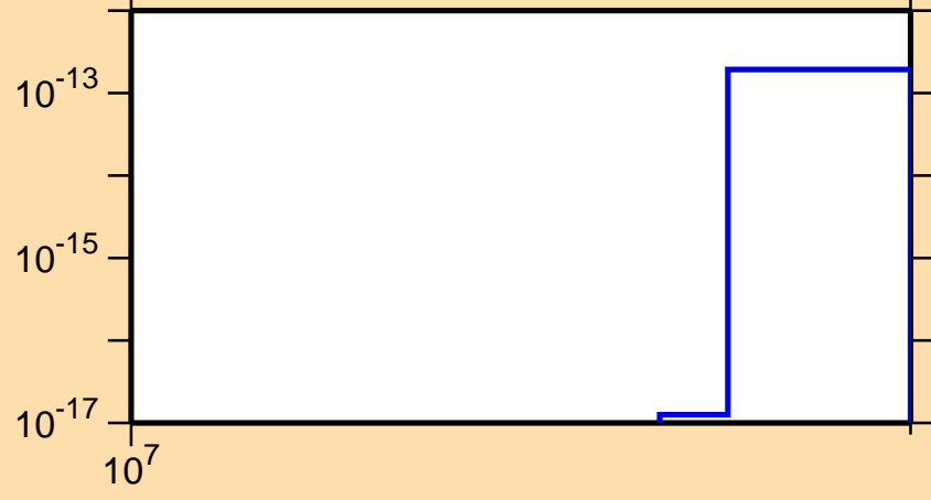
\sigma vs. E for ^{132}\text{Ce} (mt 34)
