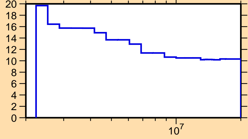
\Delta\sigma/\sigma vs. E for ^{132}\text{Ce}(n,n\text{onel.})
