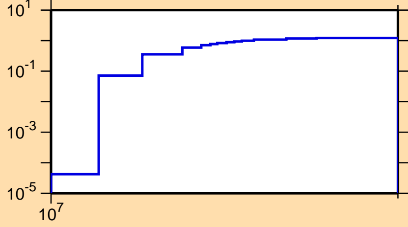
\sigma vs. E for ^{132}\text{Ce}(n,2n)
