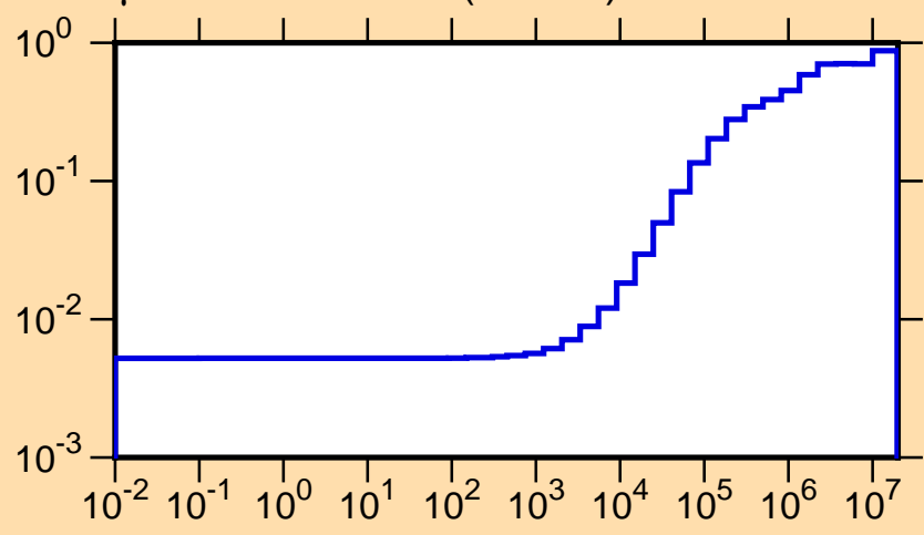
\mu vs. E for ^{132}\text{Ce}(\text{mt251})
