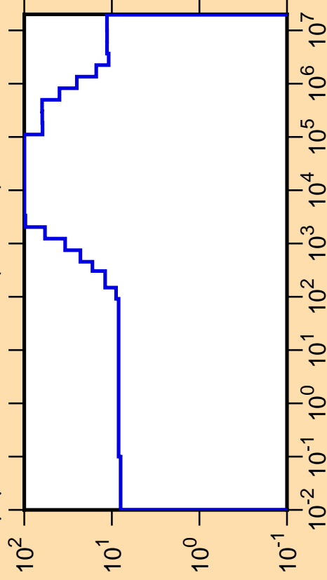
\Delta\mu/\mu vs. E for ^{132}\text{Ce}(\text{mt251})
