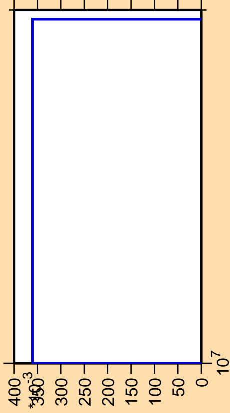
\Delta\sigma/\sigma vs. E for ^{132}\text{Ce}(n,\text{pt})
