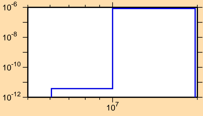
\sigma vs. E for ^{132}\text{Ce}(n,p\alpha)
