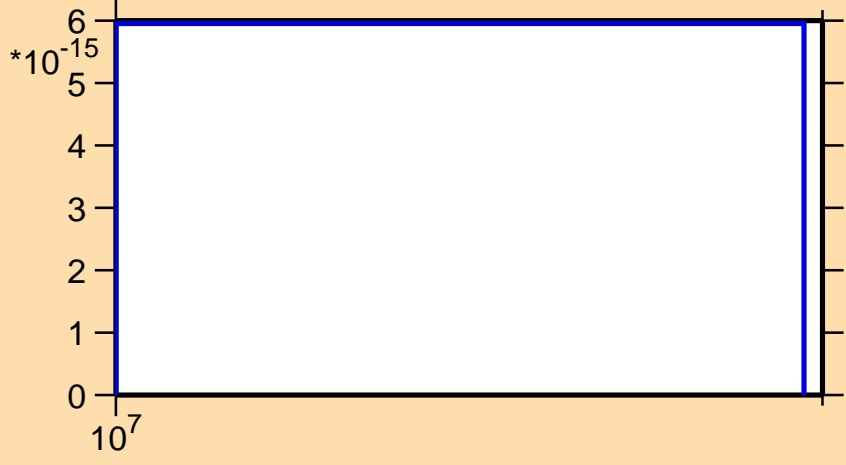
\sigma vs. E for ^{132}\text{Ce}(n,nt)
