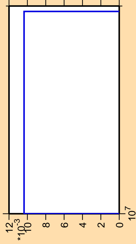
\Delta\sigma/\sigma vs. E for ^{132}\text{Ce} (mt 34)
