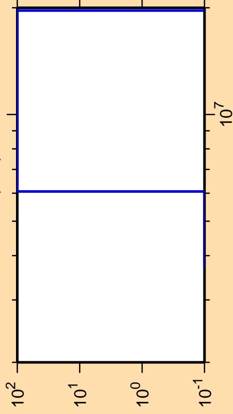
\Delta\sigma/\sigma vs. E for ^{132}\text{Ce}(n,d)
