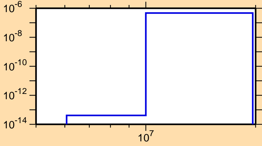
\sigma vs. E for ^{132}\text{Ce}(n,\text{He3})
