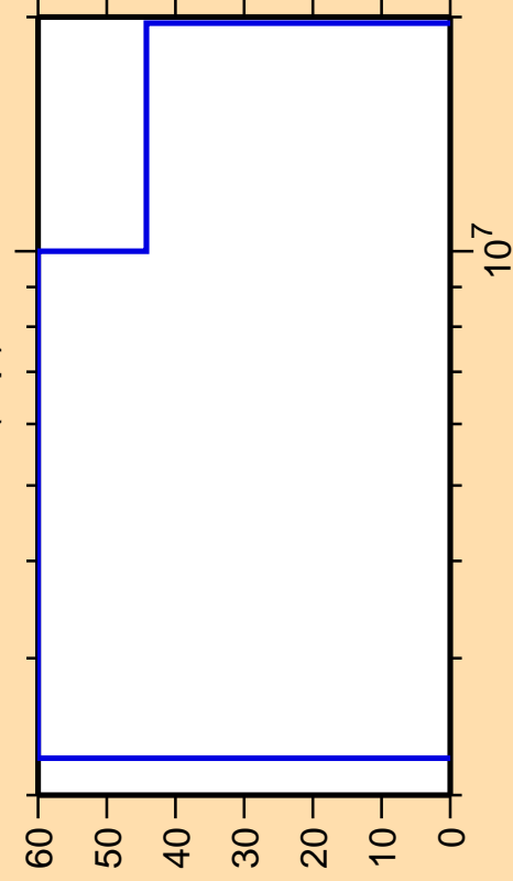
\Delta\sigma/\sigma vs. E for ^{132}\text{Ce}(n,p)
