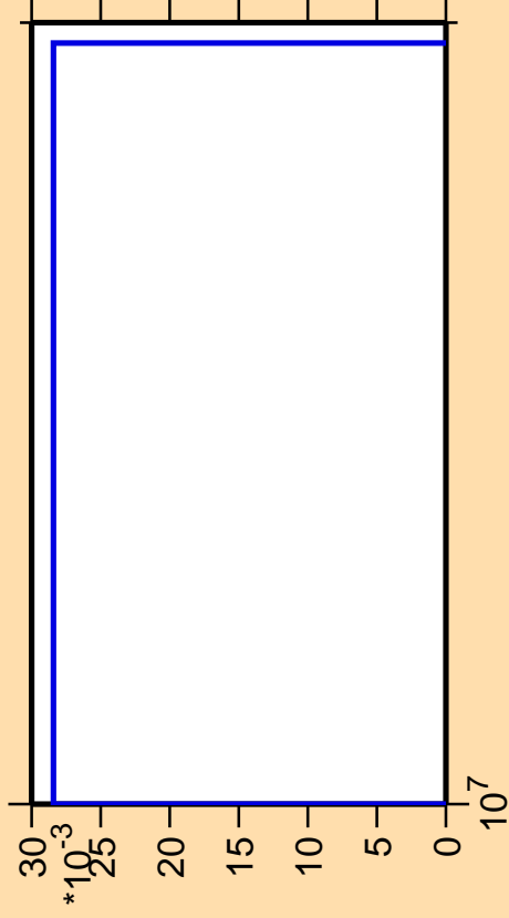
\Delta\sigma/\sigma vs. E for ^{132}\text{Ce}(n,nt)
