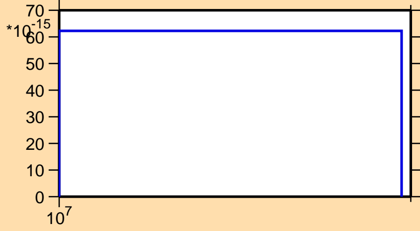
\sigma vs. E for ^{132}\text{Ce}(n,\text{pt})
