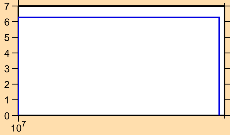
\Delta\sigma/\sigma vs. E for ^{132}\text{Ce}(n,\text{tot.})
