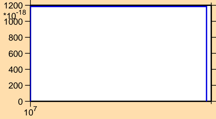
\sigma vs. E for ^{132}\text{Ce} (mt 34)
