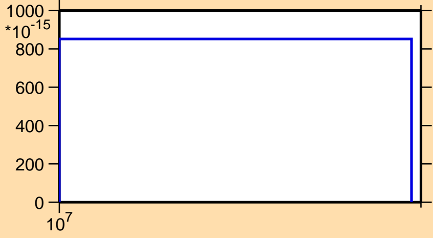
\sigma vs. E for ^{132}\text{Ce}(\text{mt117})
