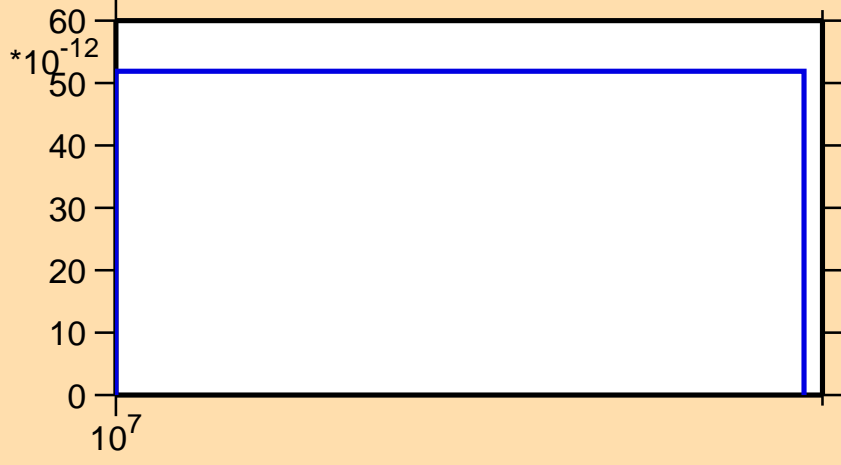
\sigma vs. E for ^{132}\text{Ce}(n,2n\alpha)
