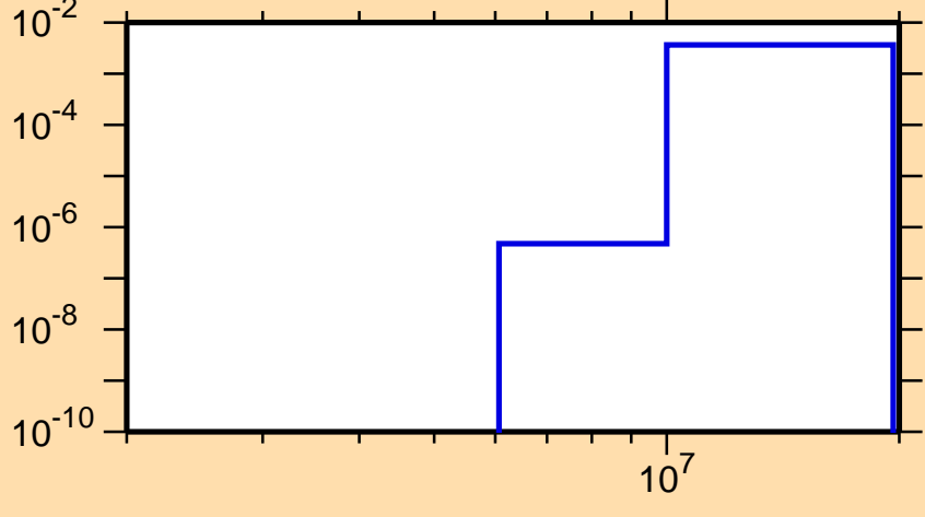
\sigma vs. E for ^{132}\text{Ce}(n,d)
