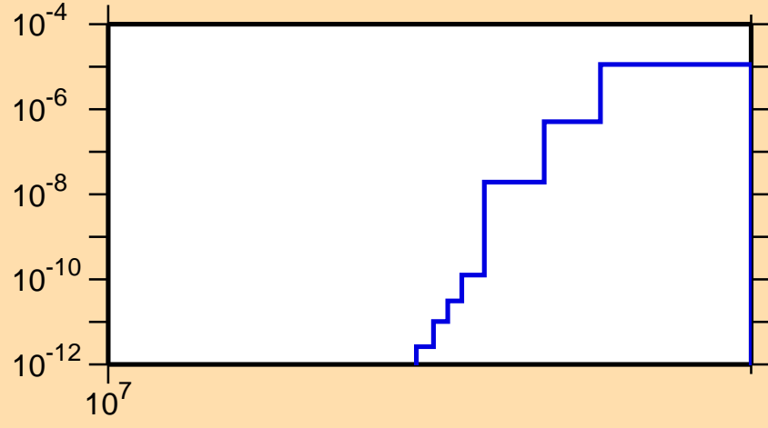
\sigma vs. E for ^{133}\text{Ce}(n,\text{nd})
