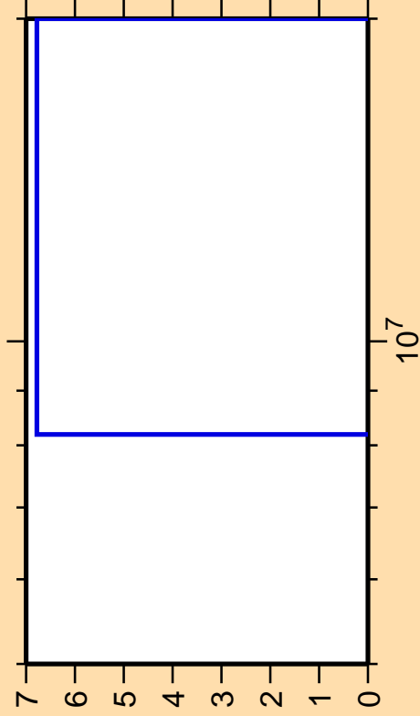
\Delta\sigma/\sigma vs. E for ^{133}\text{Ce}(\text{mt } 34)
