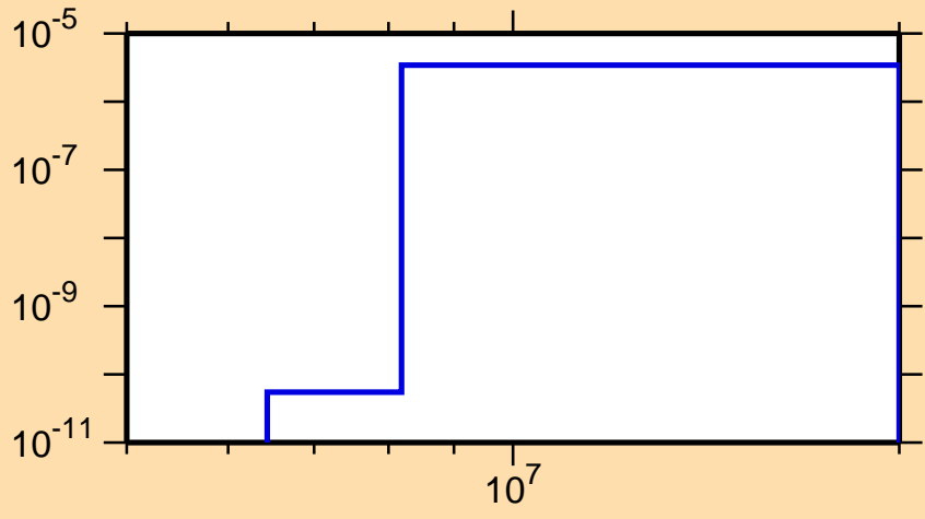
\sigma vs. E for ^{133}\text{Ce}(n,p\alpha)
