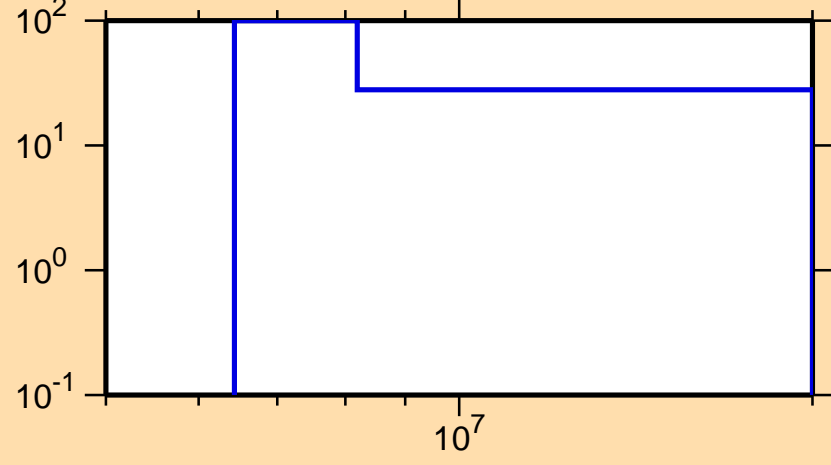
\Delta\sigma/\sigma vs. E for ^{133}\text{Ce}(n,2n)
