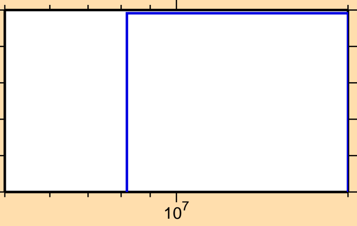
\sigma vs. E for ^{133}\text{Ce}(n,\text{He3})
