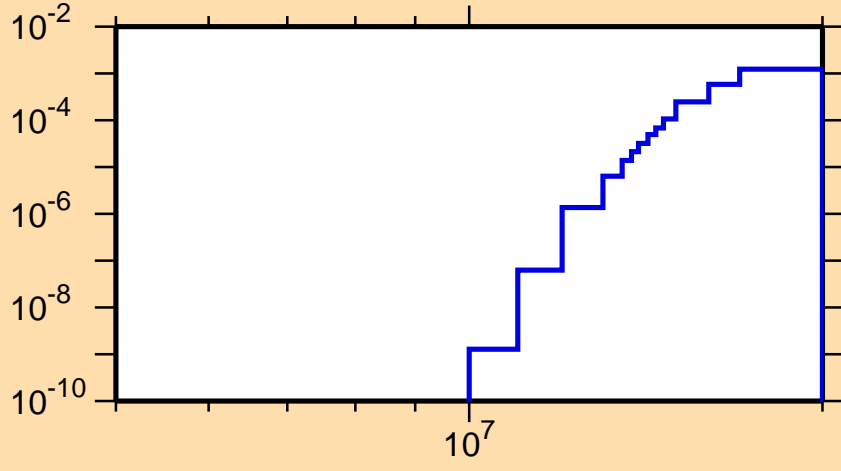
\sigma vs. E for ^{133}\text{Ce}(n,t)
