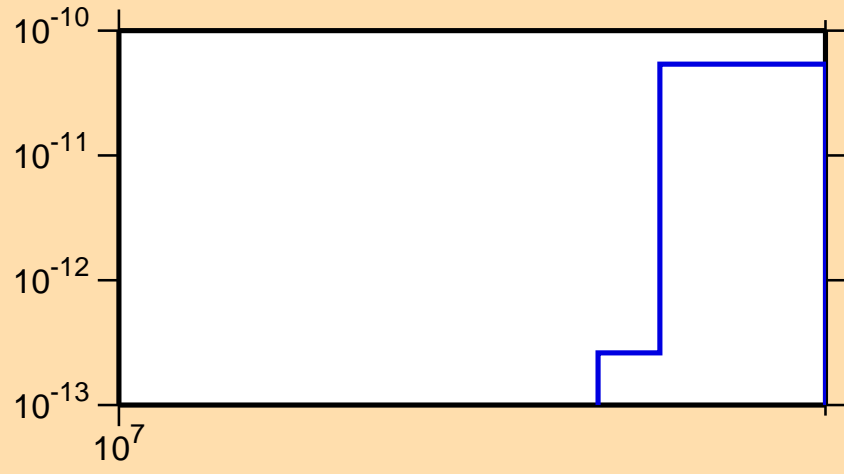
\sigma vs. E for ^{133}\text{Ce} (mt 34)
