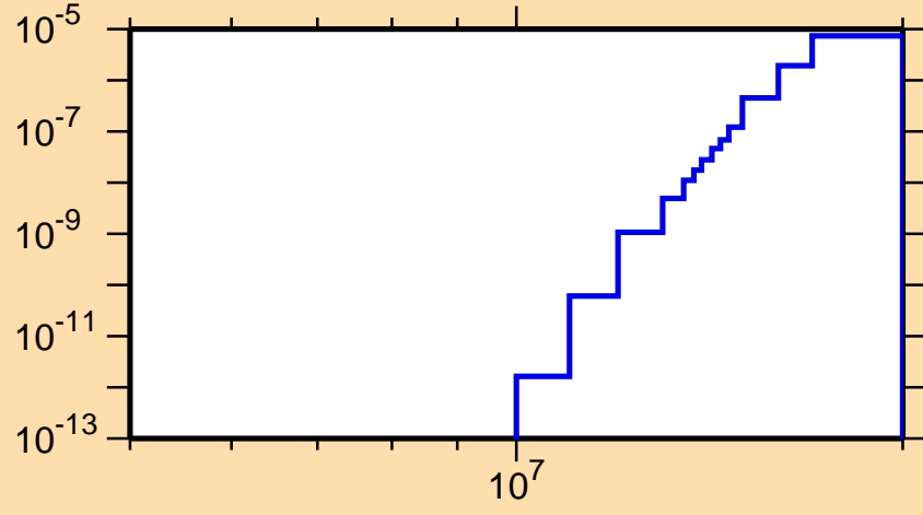
\sigma vs. E for ^{133}\text{Ce}(n,\text{He3})
