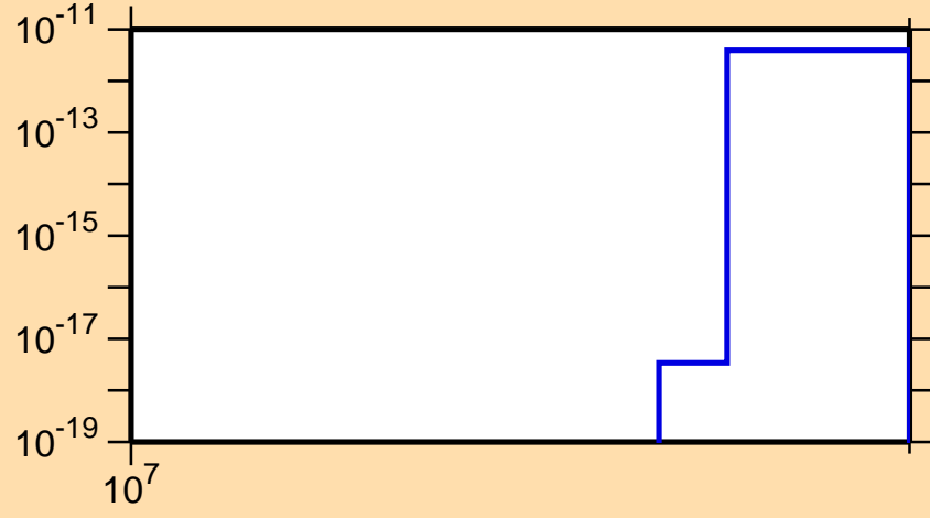
\sigma vs. E for ^{133}\text{Ce}(n,\text{nt})
