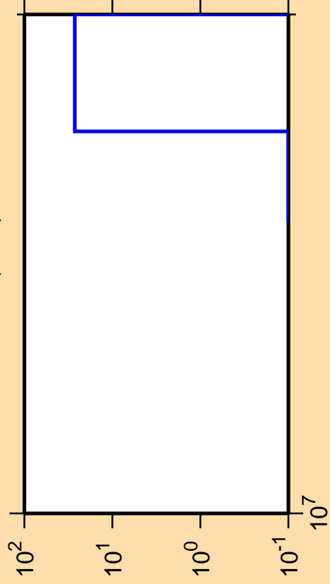
\Delta\sigma/\sigma vs. E for ^{133}\text{Ce}(n,\text{nt})
