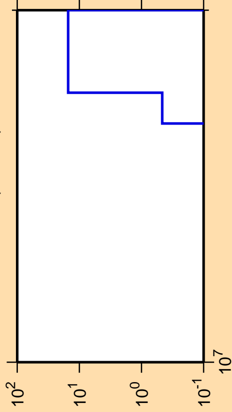
\Delta\sigma/\sigma vs. E for ^{133}\text{Ce}(\text{mt117})
