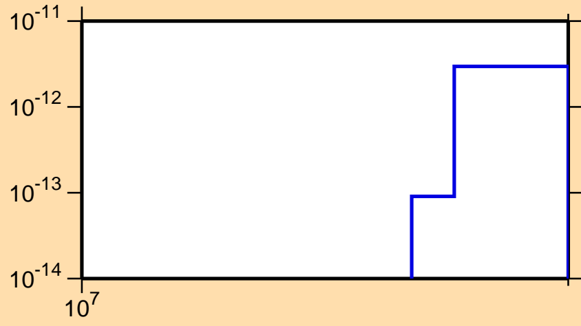
\sigma vs. E for ^{133}\text{Ce}(\text{mt117})
