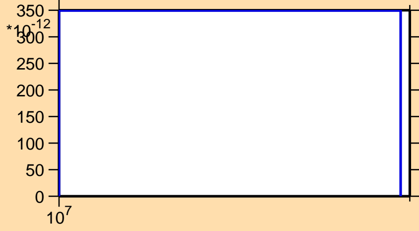
\sigma vs. E for ^{133}\text{Ce}(n,pd)
