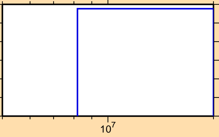
\sigma vs. E for ^{133}\text{Ce}(n,2np)
