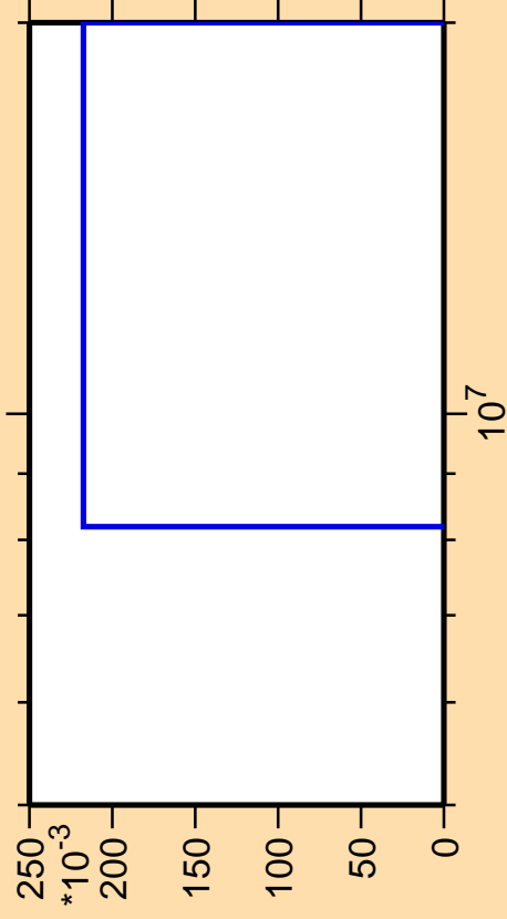
\Delta\sigma/\sigma vs. E for ^{133}\text{Ce}(n,\text{nt})
