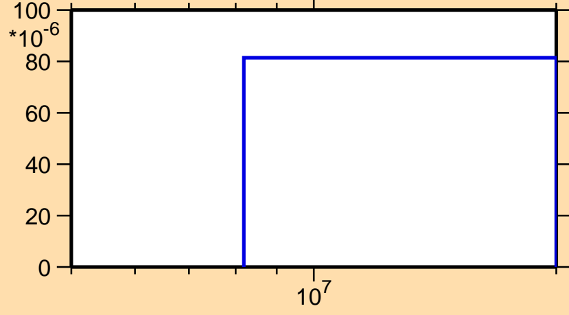
\sigma vs. E for ^{133}\text{Ce}(n,t)
