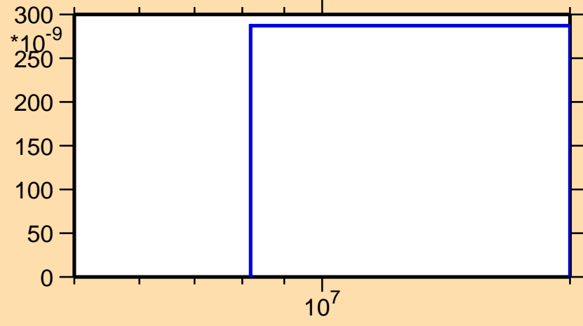
\sigma vs. E for ^{133}\text{Ce}(n,3n)
