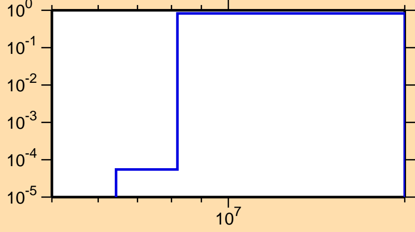
\sigma vs. E for ^{133}\text{Ce}(n,2n)
