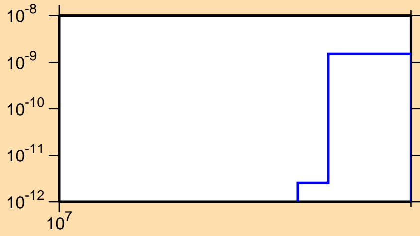
\sigma vs. E for ^{134}\text{Ce}(n,2n\alpha)
