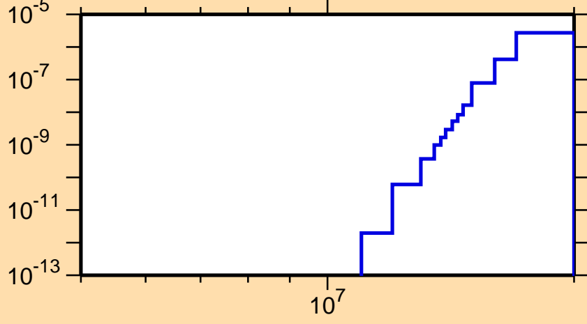
\sigma vs. E for ^{134}\text{Ce}(n,\text{He}3)
