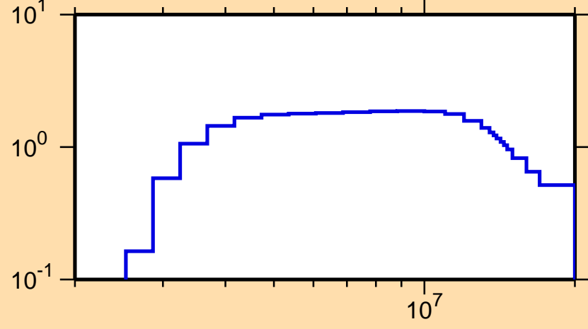
\sigma vs. E for ^{134}\text{Ce}(n,n\text{cont.})
