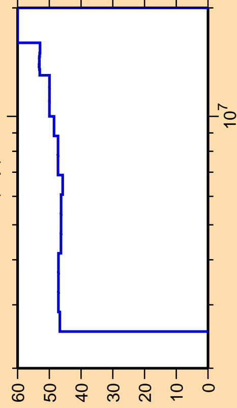
\Delta\sigma/\sigma vs. E for ^{134}\text{Ce}(n,p)
