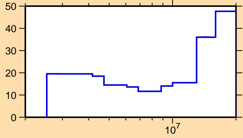
\Delta\sigma/\sigma vs. E for ^{134}\text{Ce}(n,n\text{cont.})
