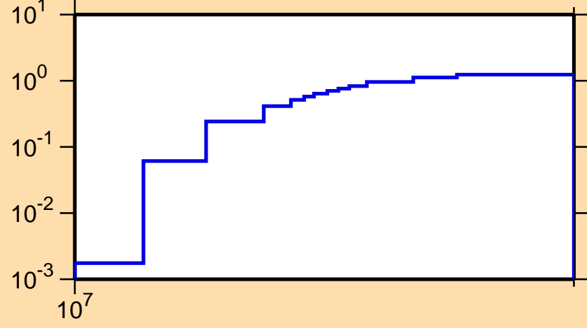
\sigma vs. E for ^{134}\text{Ce}(n,2n)
