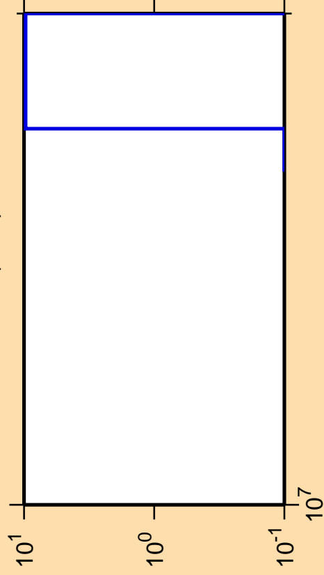
\Delta\sigma/\sigma vs. E for ^{134}\text{Ce}(n,nt)
