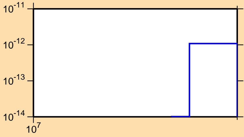
\sigma vs. E for ^{134}\text{Ce}(\text{mt117})
