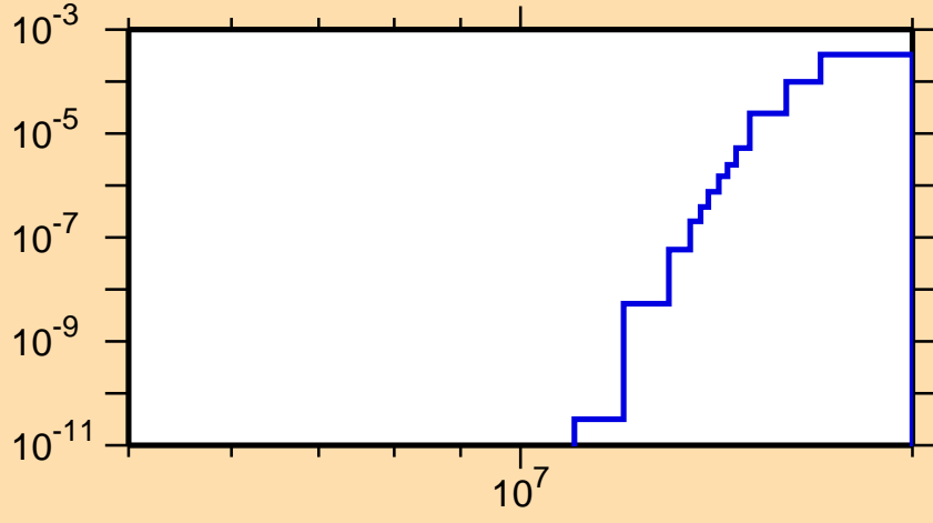
\sigma vs. E for ^{134}\text{Ce}(n,t)
