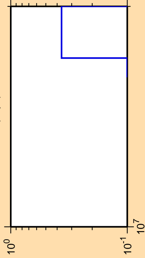
\Delta\sigma/\sigma vs. E for ^{134}\text{Ce}(n,\text{pt})
