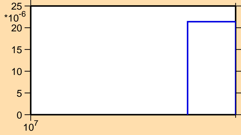
\sigma vs. E for ^{134}\text{Ce}(n,3n)
