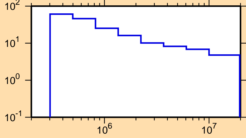
\Delta\sigma/\sigma vs. E for ^{134}\text{Ce}(n,\text{nonel.})
