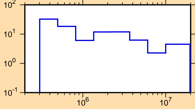
\Delta\sigma/\sigma vs. E for ^{134}\text{Ce}(n,\text{tot.})
