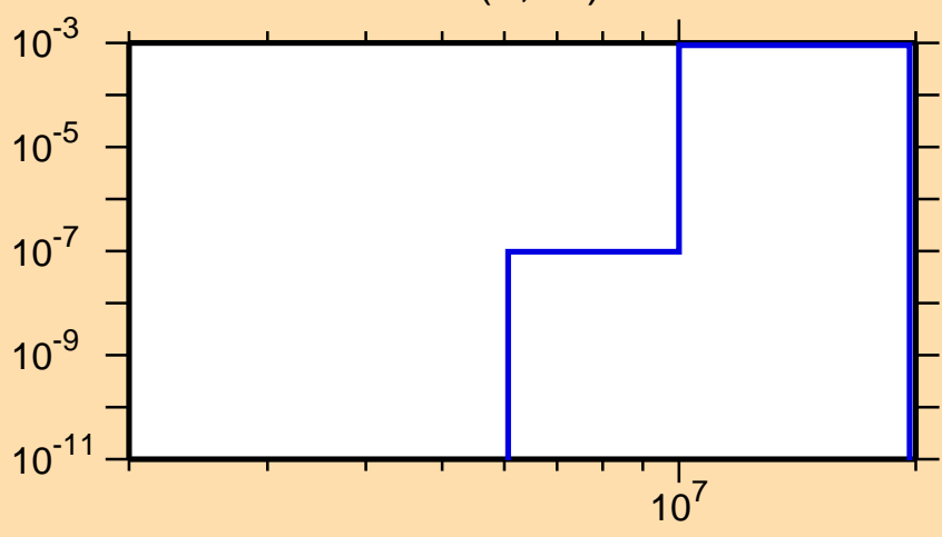
\sigma vs. E for ^{134}\text{Ce}(n,n\alpha)
