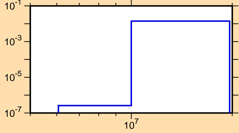
\sigma vs. E for ^{134}\text{Ce}(n,np)
