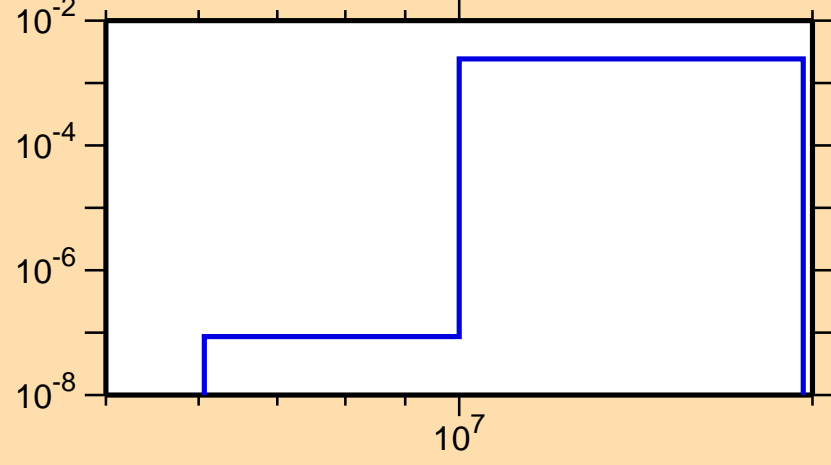
\sigma vs. E for ^{134}\text{Ce}(n,d)
