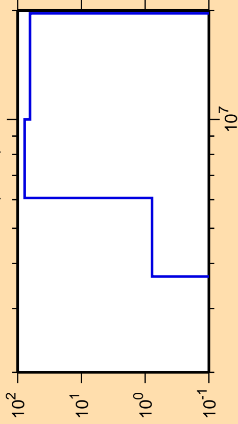
\Delta\sigma/\sigma vs. E for ^{134}\text{Ce}(n,n\alpha)
