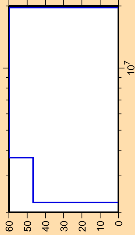
\Delta\sigma/\sigma vs. E for ^{134}\text{Ce}(n,\gamma)
