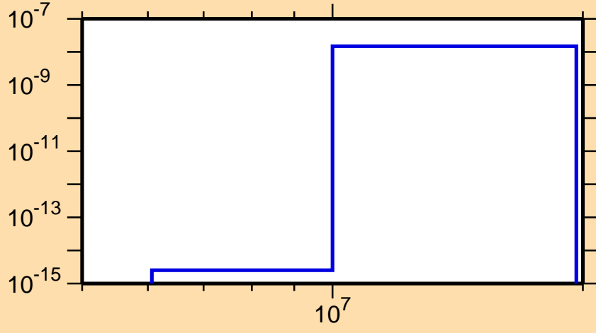
\sigma vs. E for ^{134}\text{Ce}(n,p\alpha)
