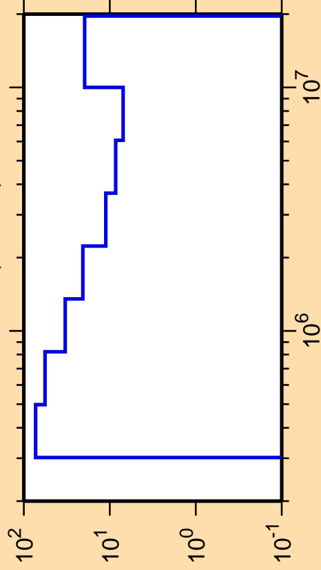
\Delta\sigma/\sigma vs. E for ^{134}\text{Ce}(n,\text{inel.})
