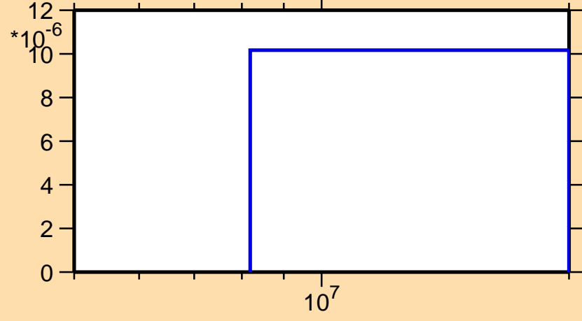
\sigma vs. E for ^{134}\text{Ce}(n,t)
