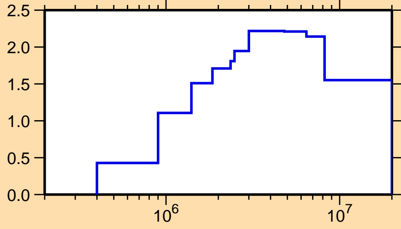
\sigma vs. E for ^{134}\text{Ce}(n,\text{inel.})
