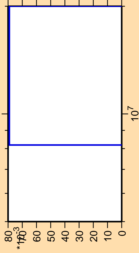
\Delta\sigma/\sigma vs. E for ^{134}\text{Ce}(n,\text{nt})
