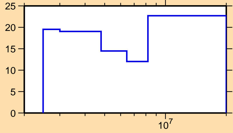
\Delta\sigma/\sigma vs. E for ^{134}\text{Ce}(n,ncont.)
