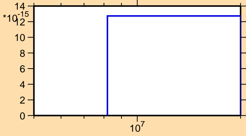
\sigma vs. E for ^{134}\text{Ce}(n,\text{nt})
