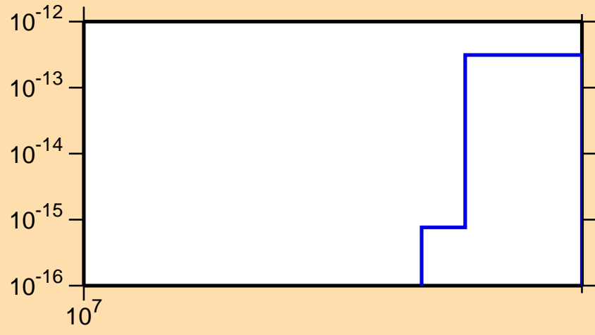
\sigma vs. E for ^{135}\text{Ce} (mt 45)
