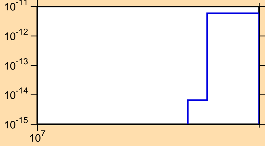
\sigma vs. E for ^{135}\text{Ce} (mt 34)
