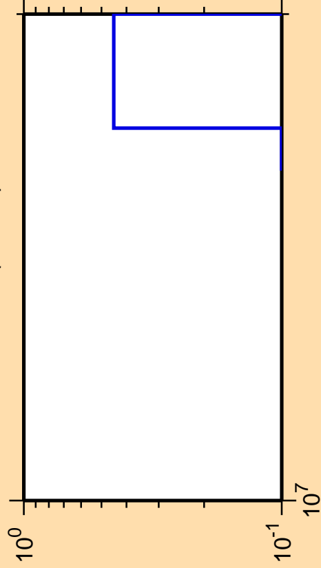
\Delta\sigma/\sigma vs. E for ^{135}\text{Ce} (mt 45)
