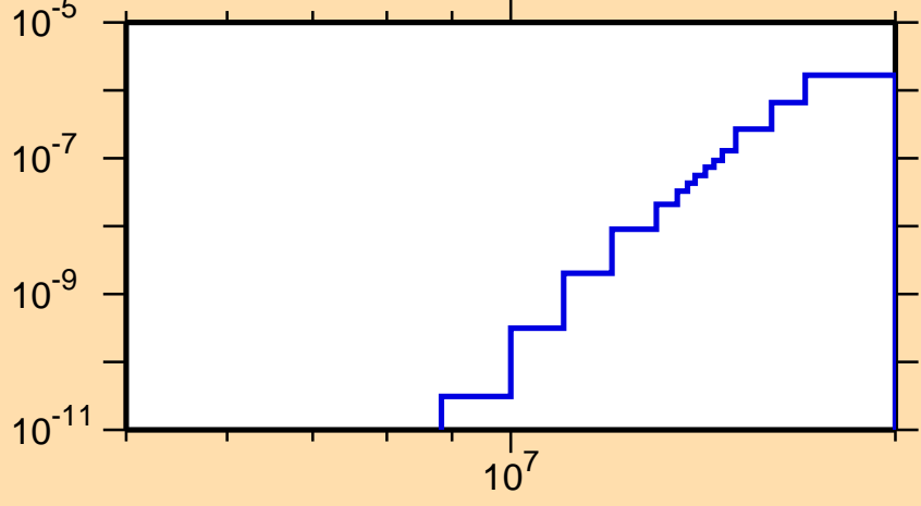
\sigma vs. E for ^{135}\text{Ce}(n,p\alpha)
