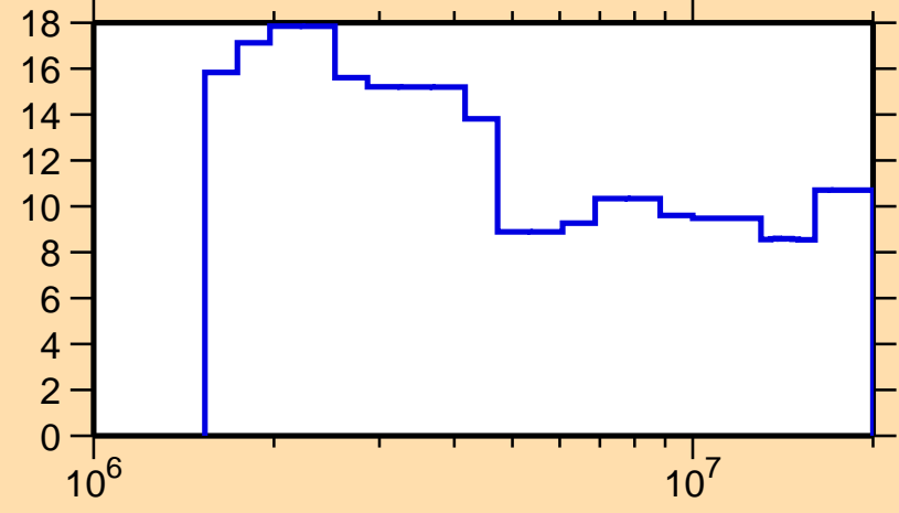
\Delta\sigma/\sigma vs. E for ^{135}\text{Ce}(n,n\text{onel.})
