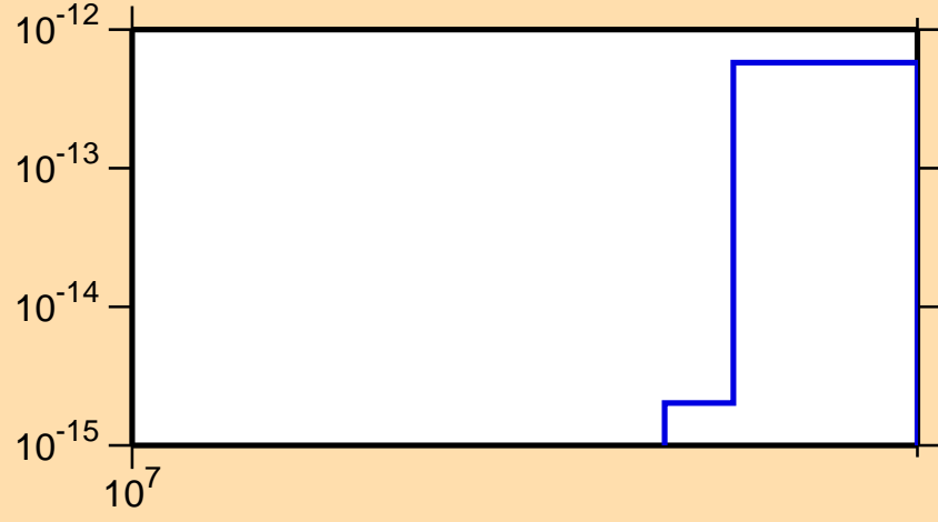
\sigma vs. E for ^{135}\text{Ce} (mt 45)
