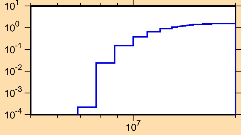
\sigma vs. E for ^{135}\text{Ce}(n,2n)
