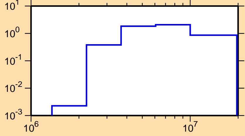
\sigma vs. E for ^{135}\text{Ce}(n,n\text{cont.})
