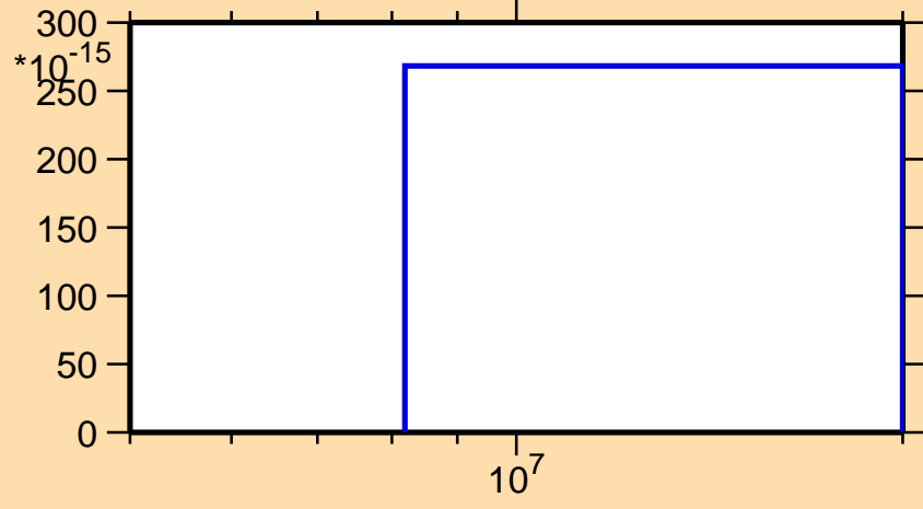
\sigma vs. E for ^{135}\text{Ce}(n,\text{nt})
