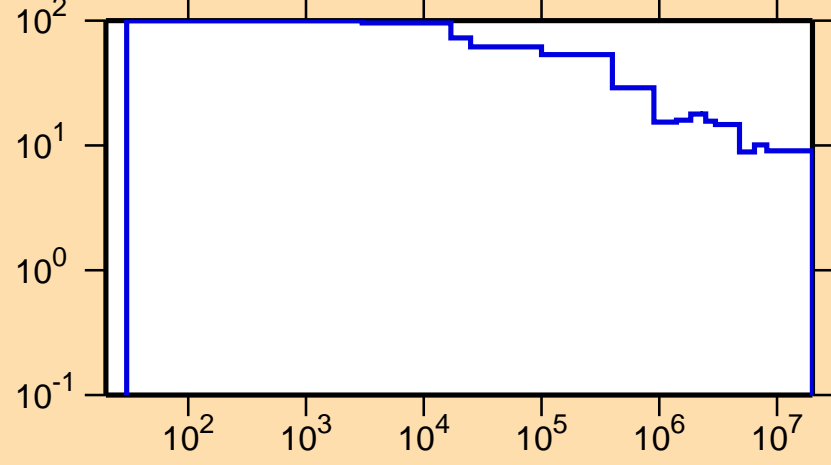
\Delta\sigma/\sigma vs. E for ^{135}\text{Ce}(n,\text{nonel.})
