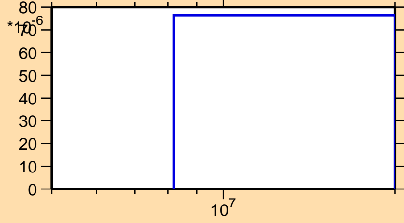
\sigma vs. E for ^{135}\text{Ce}(n,t)
