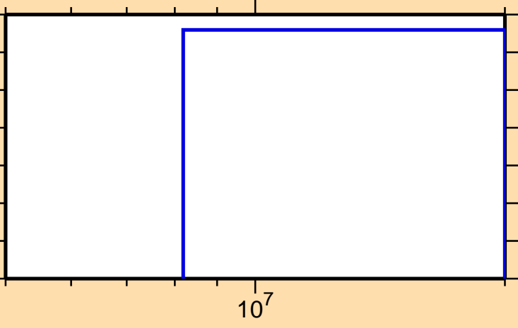
\sigma vs. E for ^{135}\text{Ce}(n,3n)
