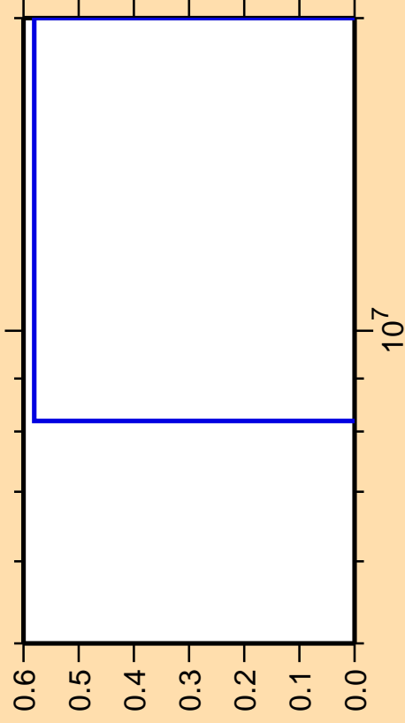
\Delta\sigma/\sigma vs. E for ^{135}\text{Ce}(n,\text{nt})
