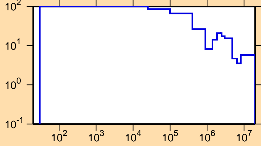
\Delta\sigma/\sigma vs. E for ^{135}\text{Ce}(n,\text{tot.})
