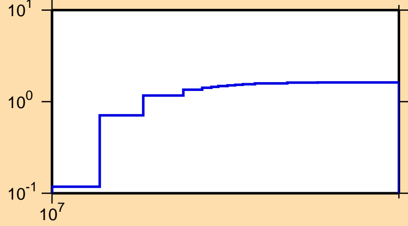
\sigma vs. E for ^{136}\text{Ce}(n,2n)
