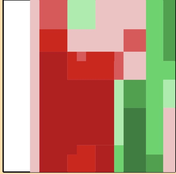
\Delta\sigma/\sigma vs. E for ^{136}\text{Ce}(n,n\text{cont.})
