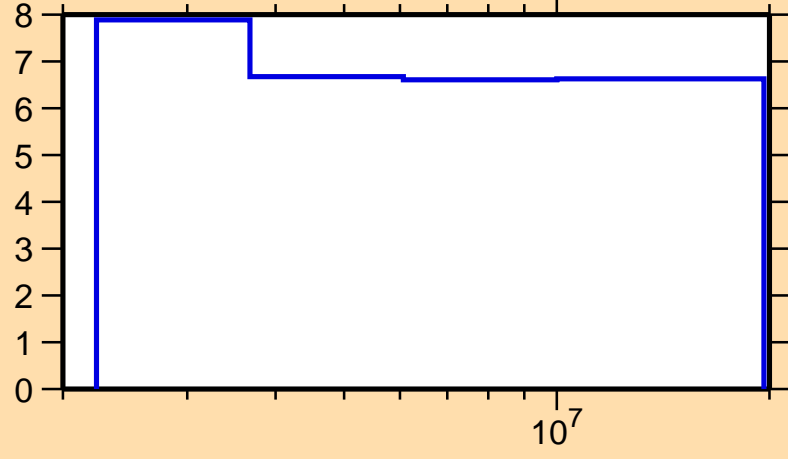
\Delta\sigma/\sigma vs. E for ^{136}\text{Ce}(n,n\text{onel.})
