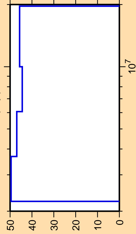
\Delta\sigma/\sigma vs. E for ^{136}\text{Ce}(n,p)
