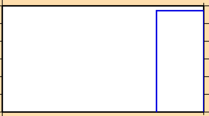
\sigma vs. E for ^{137}\text{Ce}(n,3n)
