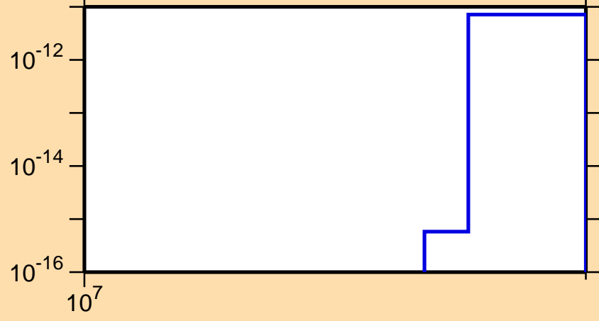
\sigma vs. E for ^{137}\text{Ce}(n,\text{pt})
