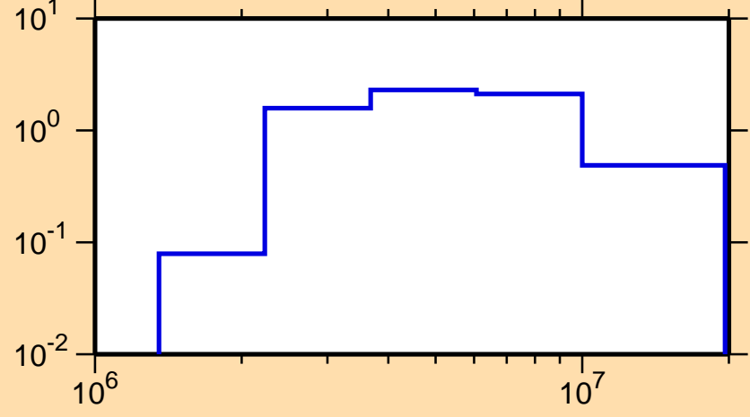
\sigma vs. E for ^{137}\text{Ce}(n,n\text{cont.})
