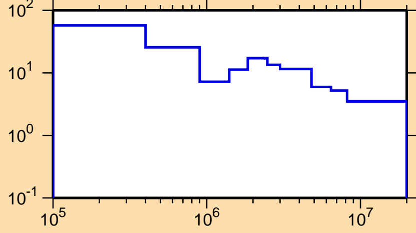
\Delta\sigma/\sigma vs. E for ^{137}\text{Ce}(n,\text{tot.})
