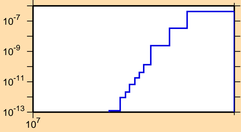
\sigma vs. E for ^{137}\text{Ce}(n,2n\alpha)
