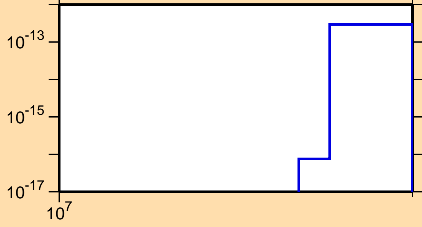
\sigma vs. E for ^{137}\text{Ce} (mt 34)
