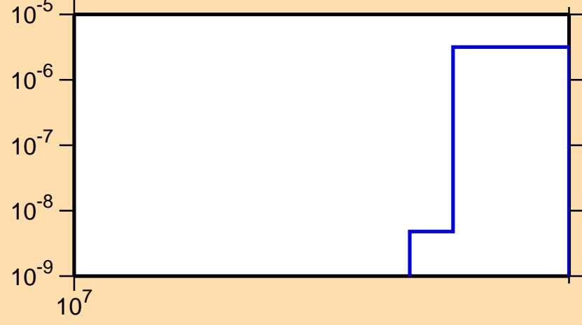
\sigma vs. E for ^{137}\text{Ce}(n,2np)
