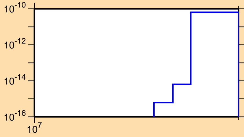
\sigma vs. E for ^{137}\text{Ce}(n,nt)
